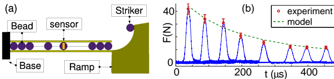
FIG. 1: (Color online) (a) Schematic diagram of the experimental setup. (b) Solitary wave decay in a chain composed of 70 steel particles impacted by a steel bead with v_{\text{imp}} = v_1 . The (blue) solid curves correspond to the recordings for sensors placed in particles 9, 16, 24, 31, 40, 50, 56, and 63.
