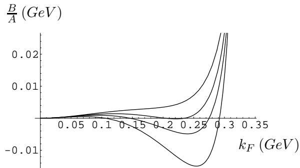
Figure 4: The binding energy, B , per nucleon in nuclear matter as a function of the Fermi momentum for various values of the scalar strength G_S . From bottom to top in the figure, the values of -G_S are (362, 340, 328, 315) \text{GeV}^{-2}
