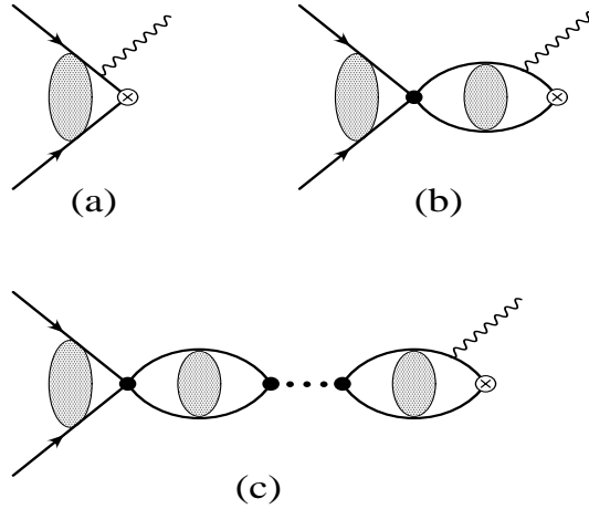
Figure 4: EFT diagrams used in order to calculate the radiative capture reaction np \rightarrow d\gamma .
