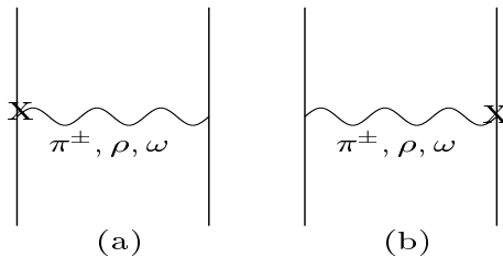
Figure 1: Parity-violating NN potential generated by meson exchange.
