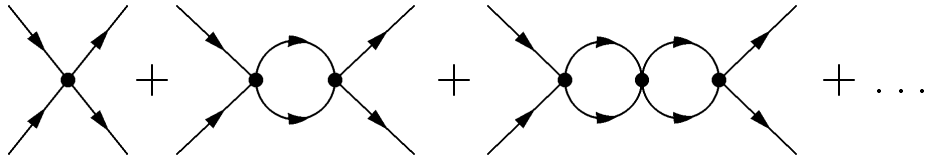
Figure 2: The multiple scattering series.
