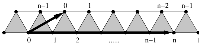
FIGURE 15. A thin torus with n points.
