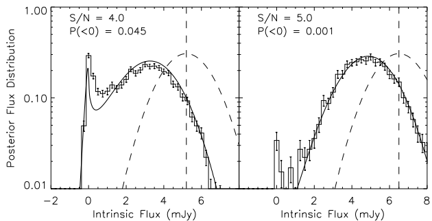
Figure 1. Posterior Flux Distribution (PFD) for S/N = 4 (left) and S/N = 5 (right) detections in a map with noise \sim 1.3 mJy assuming an underlying source population consistent with the AzTEC/COSMOS results presented in § 2.3. The simulated probability distribution is shown as the histogram and is calculated as described in § 2.1. Error bars represent the 1\sigma Poisson errors of the simulation results, limited only by the number of simulations computed. The Bayesian approximation is depicted as a solid curve. The dashed vertical line represents the measured flux, S_m . The dashed curve is the Gaussian probability distribution, p(S_m, \sigma_m | S_i) , which represents the distribution that might otherwise be assumed without flux boosting and/or false detection considerations.
