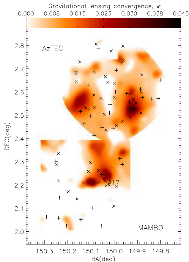
Figure 11. Weak-lensing convergence mass map (Massey et al. 2007) of the AzTEC and MAMBO surveyed regions of COSMOS. Crosses mark the millimetre source positions from the two catalogues and follow the notation of Figure 5.
