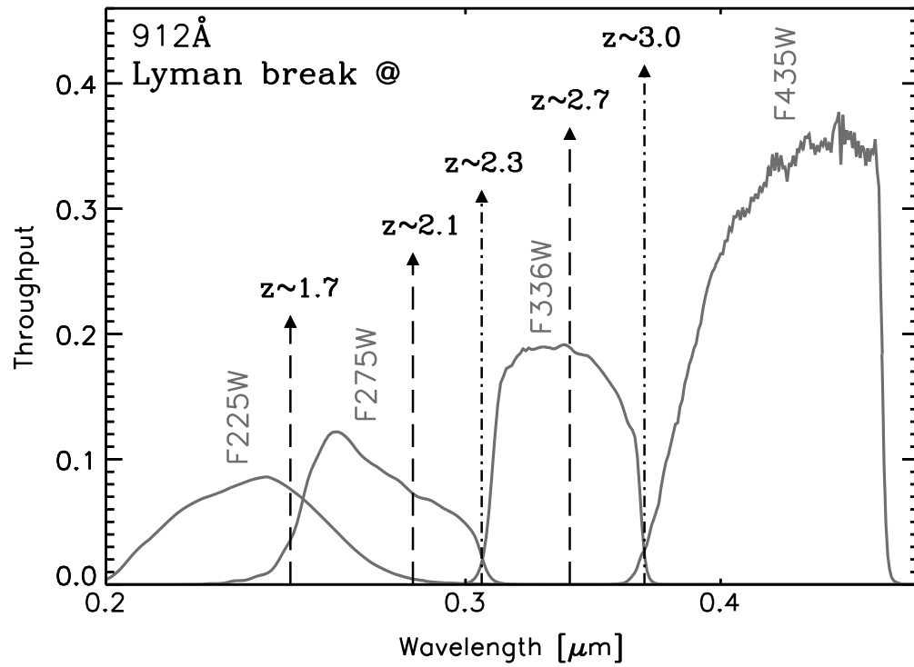
Fig. 1.— Rest-Frame 912 Å Lyman break at different redshifts is shown with filter transmission curves of three WFC3 UVIS filters and the B_{435} -band ACS optical filter. It is evident that z \simeq 1-3 LBG candidates can be efficiently selected using these three WFC3 UV filters.
