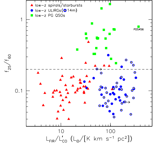
FIG. 10.— Infrared color ( f_{25}/f_{60} ) vs. L_{\text{FIR}}/L'_{\text{CO}} . The same colored symbols are used as as Figure 8. The dashed line represents f_{25}/f_{60} = 0.2 , the borderline of warm and cool ULIRGs.
