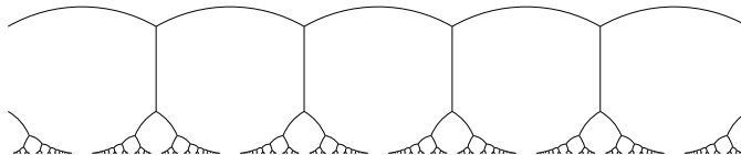
FIGURE 1. The well-rounded retract W \subset \mathfrak{H} .
