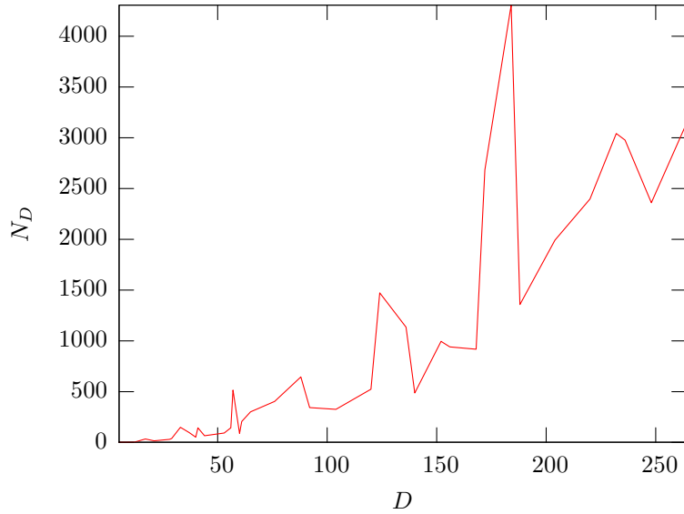
FIGURE 2. Perfect forms by discriminant
