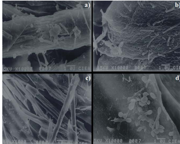
Figure 4. SEM images of feathers degradation by the mixed culture after a seven days period of petroleum removal. a), b) and d) 10,000X magnification, Bar 1.0 \mu\text{m} and c) 1,800X magnification, Bar 10.0 \mu\text{m} .
