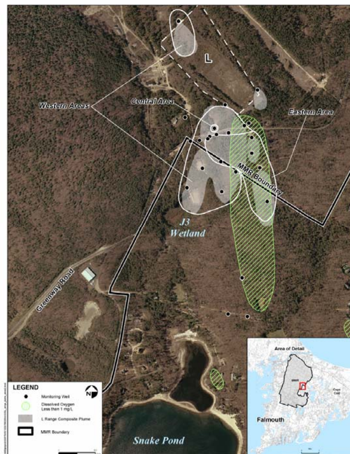
Figure 2. Location of L Range Groundwater Study Area, Factor Analysis Groundwater Zones, and anoxic zone.
