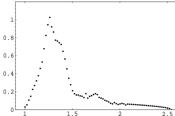
Figure 7: \bar{\rho}^{(i)}(s) vs. m_{K\pi\pi} (GeV), for i = 1 to 3 .
