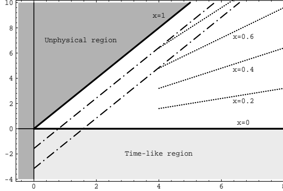
Figure 3: (\nu, Q^2) plane. Units in GeV^2 . Unshaded region is the domain of the structure functions. Solid lines are for x = 0, 0.2, 0.4, 0.6, 0.8 and 1.0 . Dashed lines are for M_R^2 = 1.6 and 3.2 GeV^2 .
