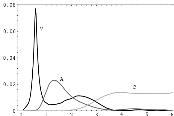
Figure 5: Vector and axial-vector spectral functions. The graph shows (V) \rho_V^R(s) , (A) \rho_A^R(s) , and (C) \rho_C(s) versus s . The s scale is given in \text{GeV}^2 .
