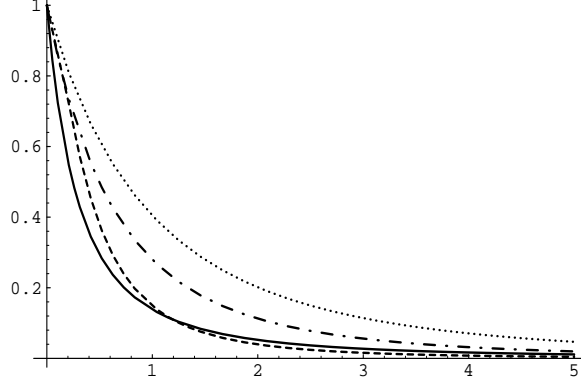
Figure 4: Factor K(\nu, s) and pion EM form factor. Pion EM form factor, solid line. K(\nu, m_\pi^2) , dashed line. K(\nu, 1 \text{ GeV}^2) , dash-dotted line. K(\nu, 2 \text{ GeV}^2) , dotted line. Horizontal scale represents Q^2 in \text{GeV}^2 .
