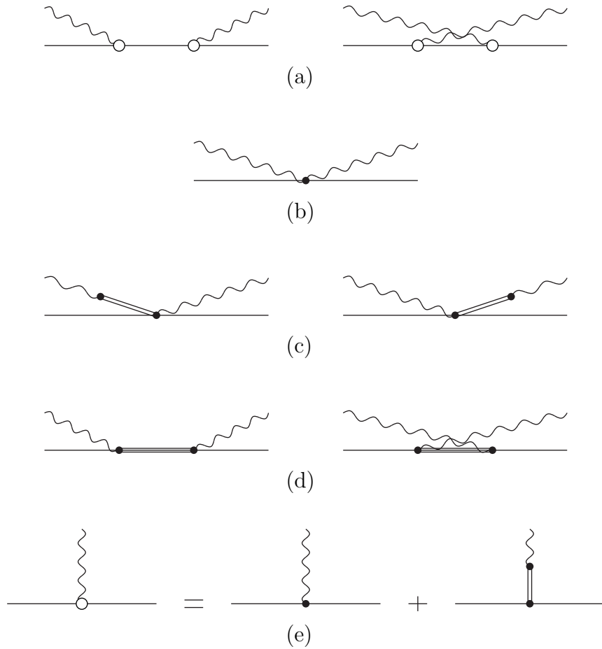
Figure 2: Compton scattering diagrams for the meson resonances. (a) Elastic diagram. (b) Pseudoscalar seagull diagram. (c) Vector resonance seagull diagram. (d) Axial-vector resonance intermediate state diagram. (e) Pion form factor diagrams.
