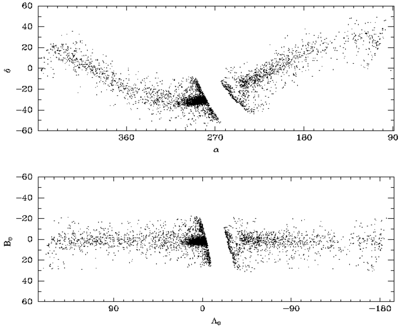
Fig. 12.— The -7 < Z_{Sgr,GC} < 7 kpc sample explored in Figure 13 shown in equatorial and Sgr coordinates.
