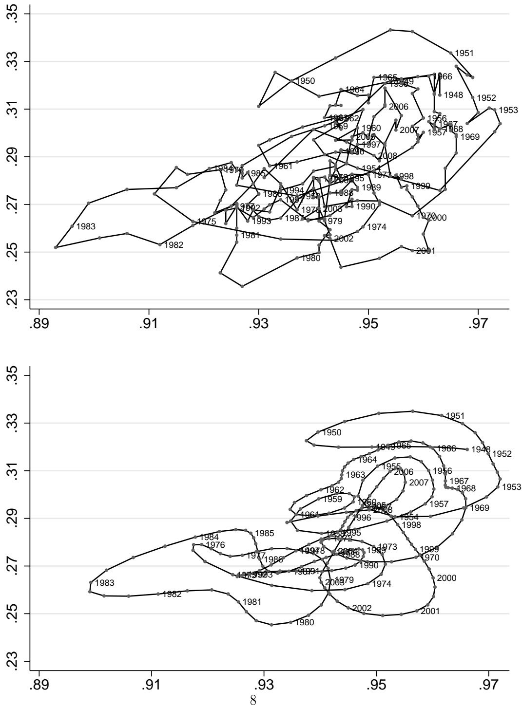
FIGURE 7 - US actual and smoothed (e, \pi) -plane cycles
