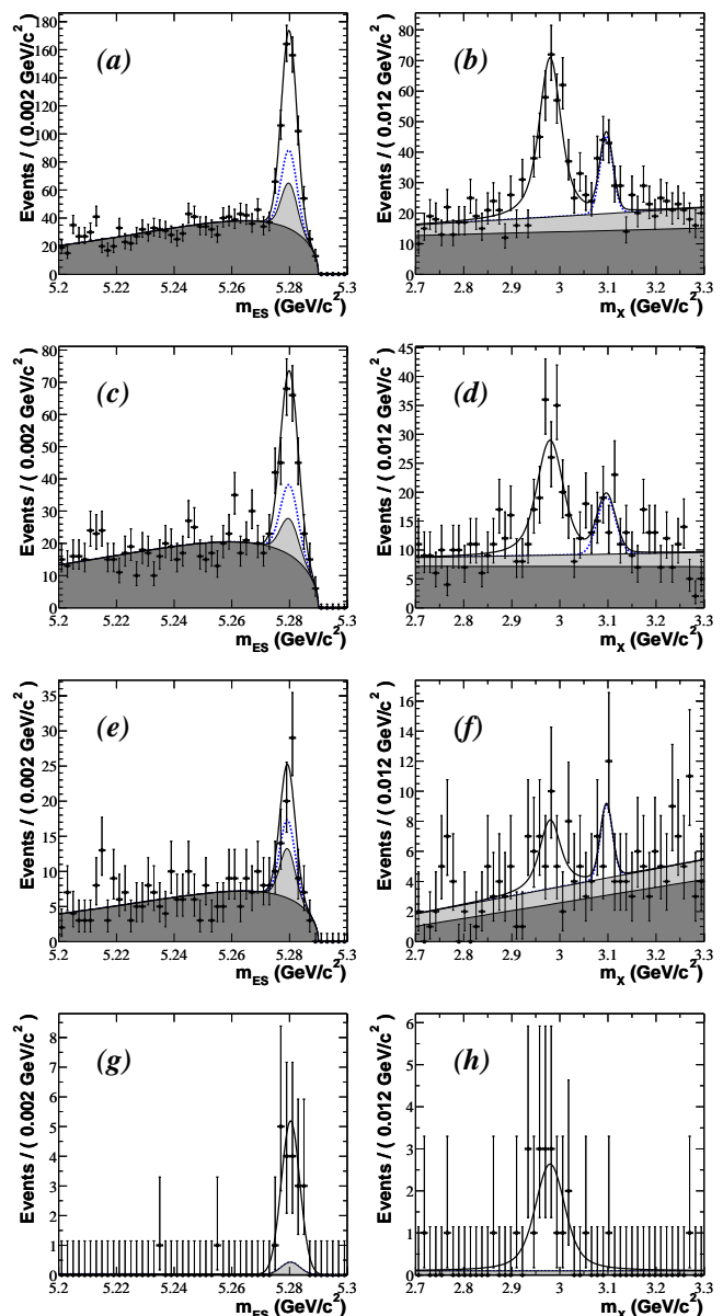
FIG. 1: Distributions of m_{ES} (left) and m_X (right) for charged B candidates. The m_{ES} distributions displayed here are restricted to the 2.90 < m_X < 3.15 \text{ GeV}/c^2 range; similarly, the m_X distributions include only events in the m_{ES} signal region ( m_{ES} > 5.27 \text{ GeV}/c^2 ). Each pair corresponds to a different \eta_c decay mode: (a, b) \eta_c \rightarrow K_S^0 K^\pm \pi^\mp ; (c, d) \eta_c \rightarrow K^+ K^- \pi^0 ; (e, f) \eta_c \rightarrow 2(K^+ K^-) ; and (g, h) \eta_c \rightarrow \phi\phi . The fitted p.d.f. projections are shown as solid curves. In each plot, the dark grey region corresponds to the combinatorial background component, light grey highlights the peaking background, and the dotted line is the sum of the total background and of the J/\psi component.
