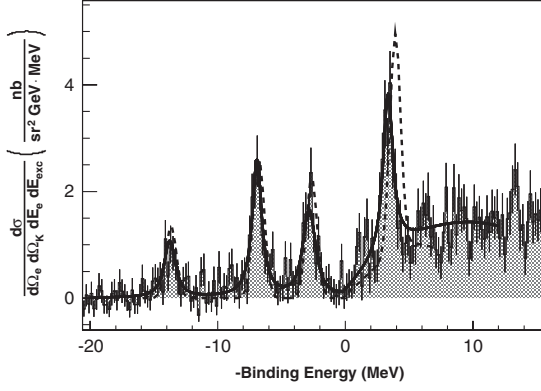
FIG. 3. The {}^{16}_{\Lambda}\text{N} binding-energy spectrum. The best fit using Voigt functions (solid curve) and a theoretical prediction (dashed curve) are superimposed on the data. See text for details.
