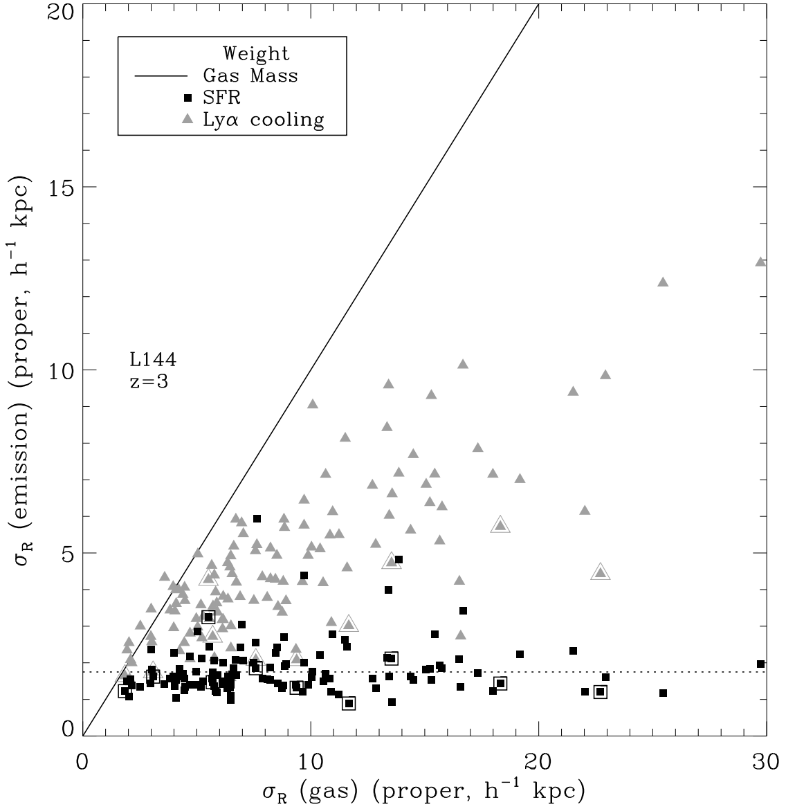
Fig. 5.— Radial rms extent of the gas in the cooling groups at z = 3 , weighted by several different factors. The x -axis is weighted by the gas mass. On the y -axis, the triangles are weighted by the \text{Ly}\alpha emission (considering only the “gravitational” cooling). The squares are weighted by the star formation rate, which is proportional to the stellar ionizing emission. The dotted line shows the gravitational softening length. The points would lie on the solid line if the emissivity were proportional to the gas density. Only groups with \text{Ly}\alpha cooling of more than 10^{43} \text{ erg s}^{-1} are shown; groups with \text{Ly}\alpha cooling of more than 5 \times 10^{43} \text{ erg s}^{-1} are shown surrounded by outlines.
