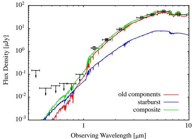
FIG. 5.— Synthetic SEDs of old stellar components (red), starburst components at the age of 100 Myr with an initial SFR of 3000 M_{\odot} \text{ yr}^{-1} (blue), and a sum of both (green) created with the GALAXEV library. Photometry data are also shown.
