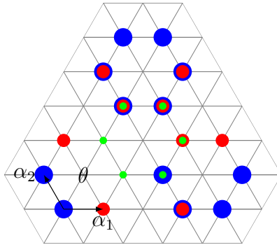
Figure 10: The support of the numerator of Z^*(\mathbf{X}; \mathbf{m})
