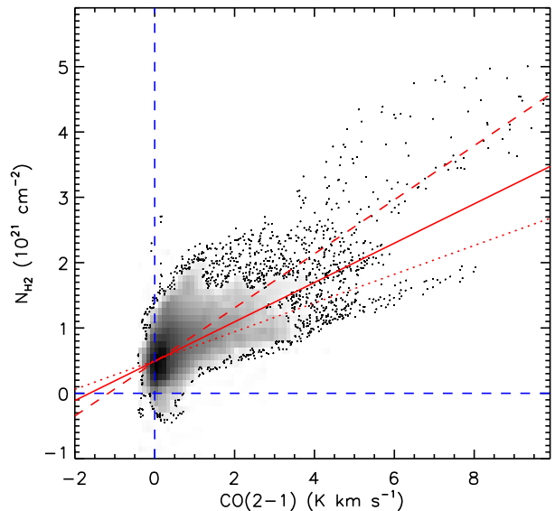
Fig. 5. Scatter plot of H_2 column density as derived from the dust emission and the \text{CO}(2-1) intensity. The solid red line is a fit to the entire dataset and corresponds to a N(H_2)/I_{CO(2-1)} value of 3 \times 10^{20} \text{ H}_2 \text{ per K km s}^{-1} with an offset as described in the text. A radial variation is present: fitting within 2 kpc yields a N(H_2)/I_{CO(2-1)} value of 2.2 \times 10^{20} \text{ H}_2 \text{ per K km s}^{-1} and 4.1 \times 10^{20} \text{ H}_2 \text{ per K km s}^{-1} beyond 2 kpc (dotted and dashed lines, respectively).
