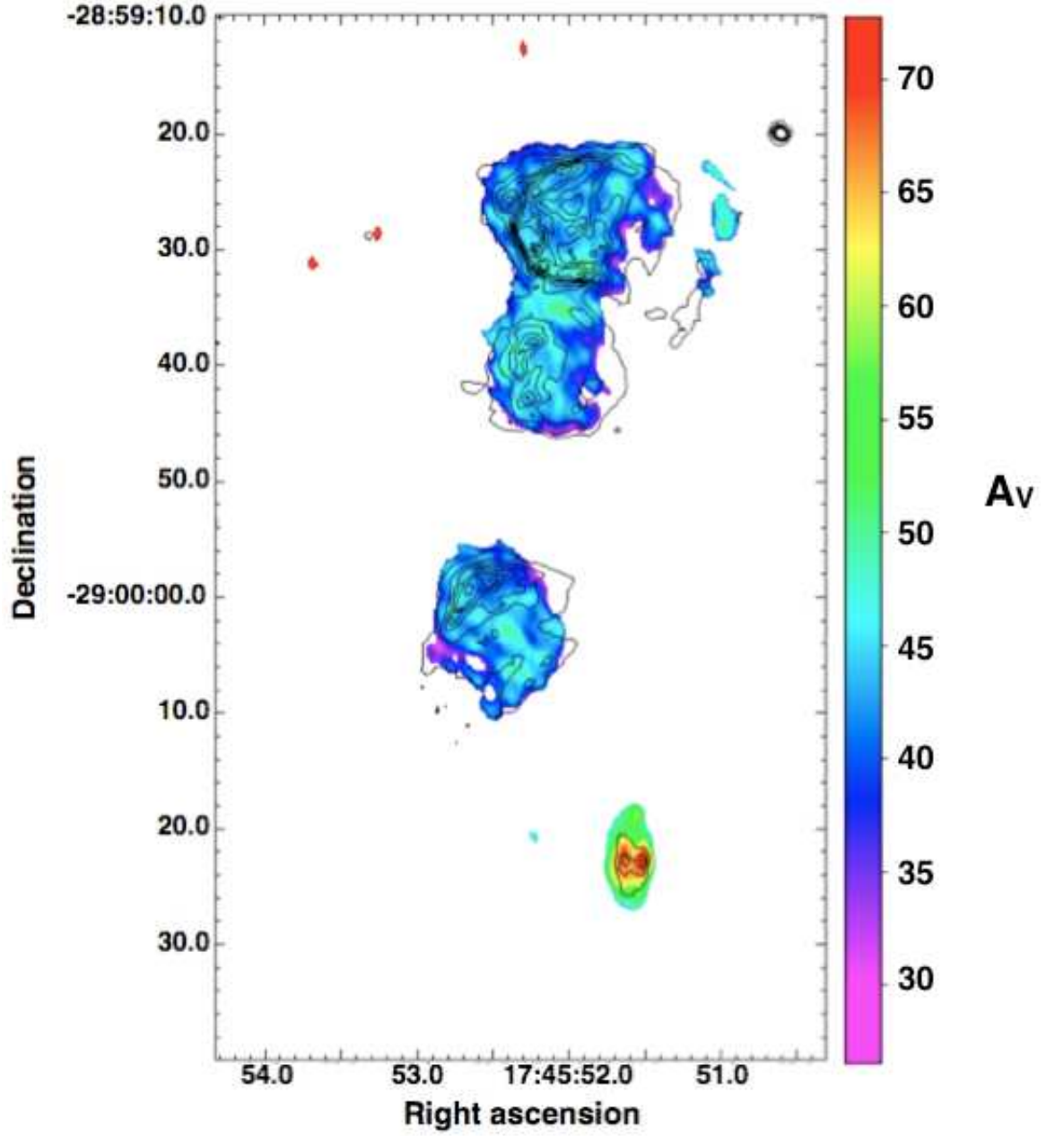
FIG. 5.— Map of the extinction toward the HII regions G-0.02-0.07 derived from a comparison between P\alpha and 8.4 GHz continuum data. The resolution of the map is the same as the 8.4 GHz data, or 1.5 \times 0.8 arcseconds. The contours represent the flux density of the smoothed P\alpha emission. The lowest contour has a values of 0.5 \text{ mJy per arcsec}^{-2} , and the contours are spaced by 0.8 \text{ mJy per arcsec}^{-2} .
