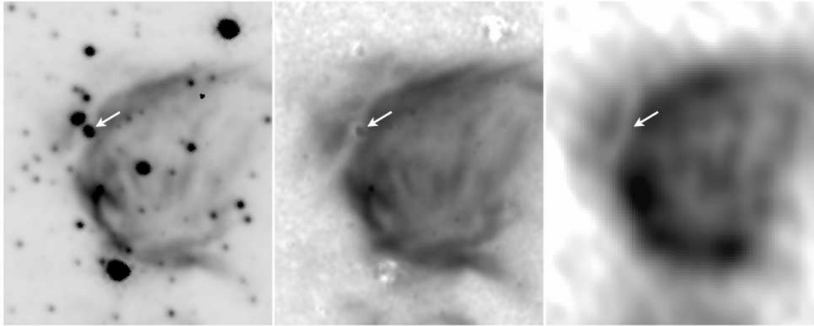
FIG. 9.— A comparison of the emission toward the northeast extension of region A from the F187N filter, the pure P\alpha line image, and the 8.4 GHz radio image, from left to right. An emission-free lane is seen separating the main shell of region A from a slight extension at the 10 o'clock position. Like region D, there is a star apparently located slightly offset from the center of this lane ( its location indicated in all images with an arrow). The apparent P\alpha excess at the position of this star is at has the same intensity as the emission from the surrounding nebula, and is likely an artifact due to the difficulty of subtracting stellar emission in the presence of a diffuse background. No counterpart to the apparent P\alpha excess at the position of this star is seen in the radio image. In images of Cotera et al. (2000), this star appears highly reddened, but its H-K' color is not given.
