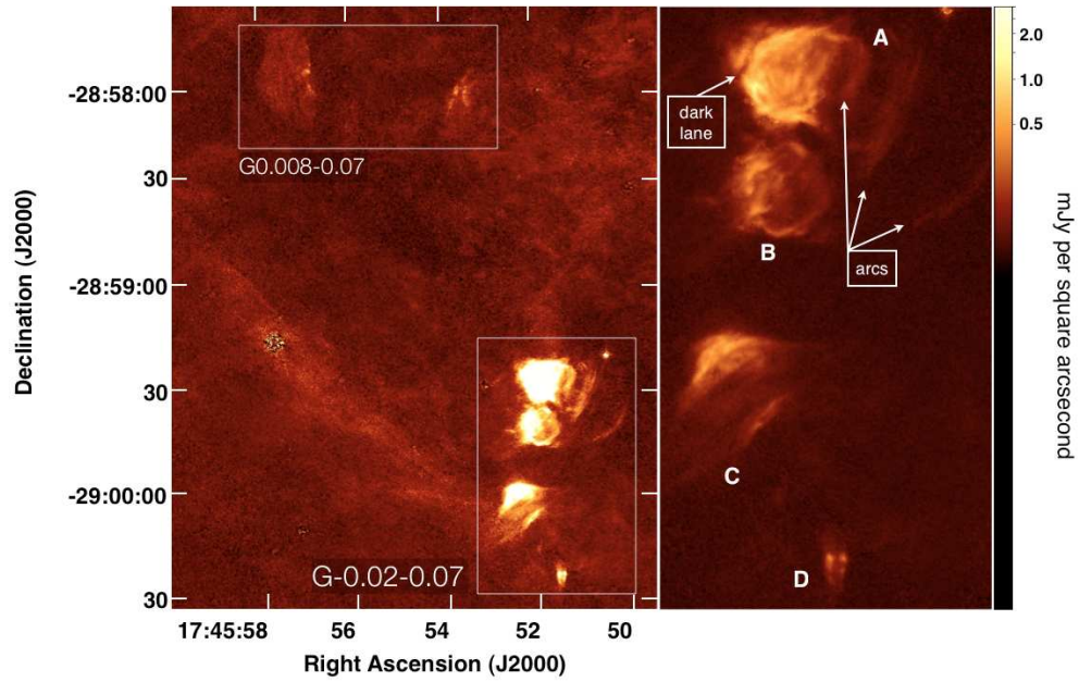
FIG. 2.— Left: P\alpha image showing a view of the G-0.02-0.07 HII regions (from top to bottom: A,B,C and D) and their surroundings, including a bright emission line star located to the northwest of region A. A ridge of emission can be seen, which appears to emanate from region C, and extend up to the northeast. Visible in the box to the upper left is the newly discovered HII region G0.008-0.07. Right: An enlarged view of the G-0.02-0.07 HII regions, the focus of this paper, with a stretch chosen to enhance the various filamentary features visible in the P\alpha image. Regions A through D are individually labeled, as are several features of interest, including a dark lane separating region A from a slight extension to the northeast, and a series of filaments extending outward from the West side of region A.
