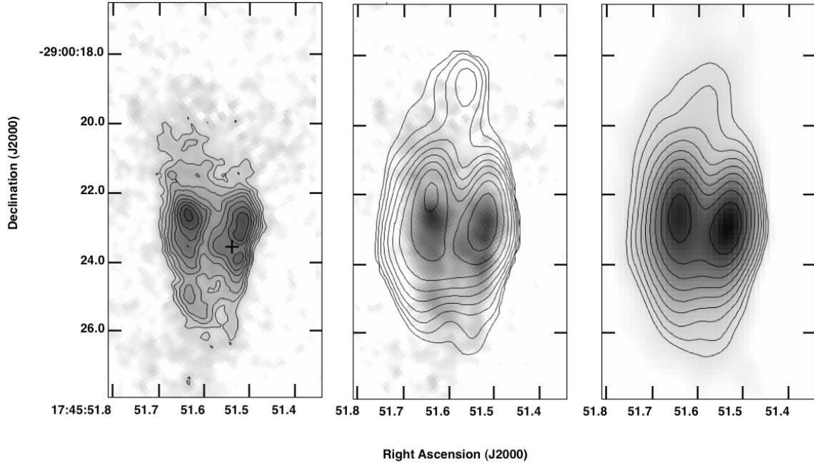
FIG. 6.— Detail maps of the structure of region D in pure Paschen alpha line emission, with contours of flux density (Left) and extinction (Center) overlaid. For comparison, the 8.4 GHz image of region D is also shown (Right). On the Left, the flux density contours have a logarithmic spacing, with the lowest contour having a value of 0.5 \text{ mJy per arcsec}^{-2} , and the highest having a value of 3 \text{ mJy per arcsec}^{-2} . The cross marks the position of the star seen in Figure 7. In the Center, the lowest and highest extinction contours correspond to values of A_V = 50 and 70 , respectively, with a contour spacing of 2.5 magnitudes. On the Right, the contours on the radio image are logarithmically spaced, with the lowest contour corresponding to a flux density of 0.5 \text{ mJy} and the highest corresponding to 20 \text{ mJy} .
