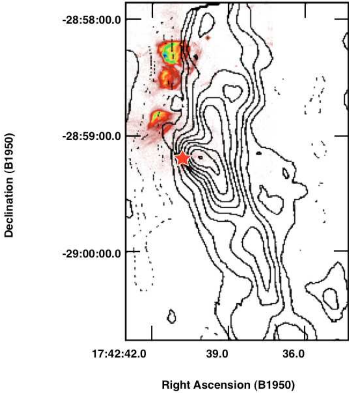
FIG. 10.— Superposition of Ammonia (1,1) contours (Coil & Ho 2000, magnification of their Figure 6, Left) and P\alpha emission, showing the apparent association of region D (indicated with a star) with a dense core in the western ridge of M-0.02-0.07. Region D appears to be immediately adjacent to a steep gradient in the ammonia emission from the core.
