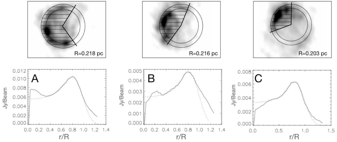
FIG. 4.— Top: Projected shells (with outer radius size indicated for each shell) are superposed on the 8.44 GHz images used to fit shell parameters. Bottom: Azimuthally-averaged radial profiles for each HII region are shown (solid lines). A shell model of the emission measure (dotted lines) is fit to each HII region, from which the electron density can be derived.
