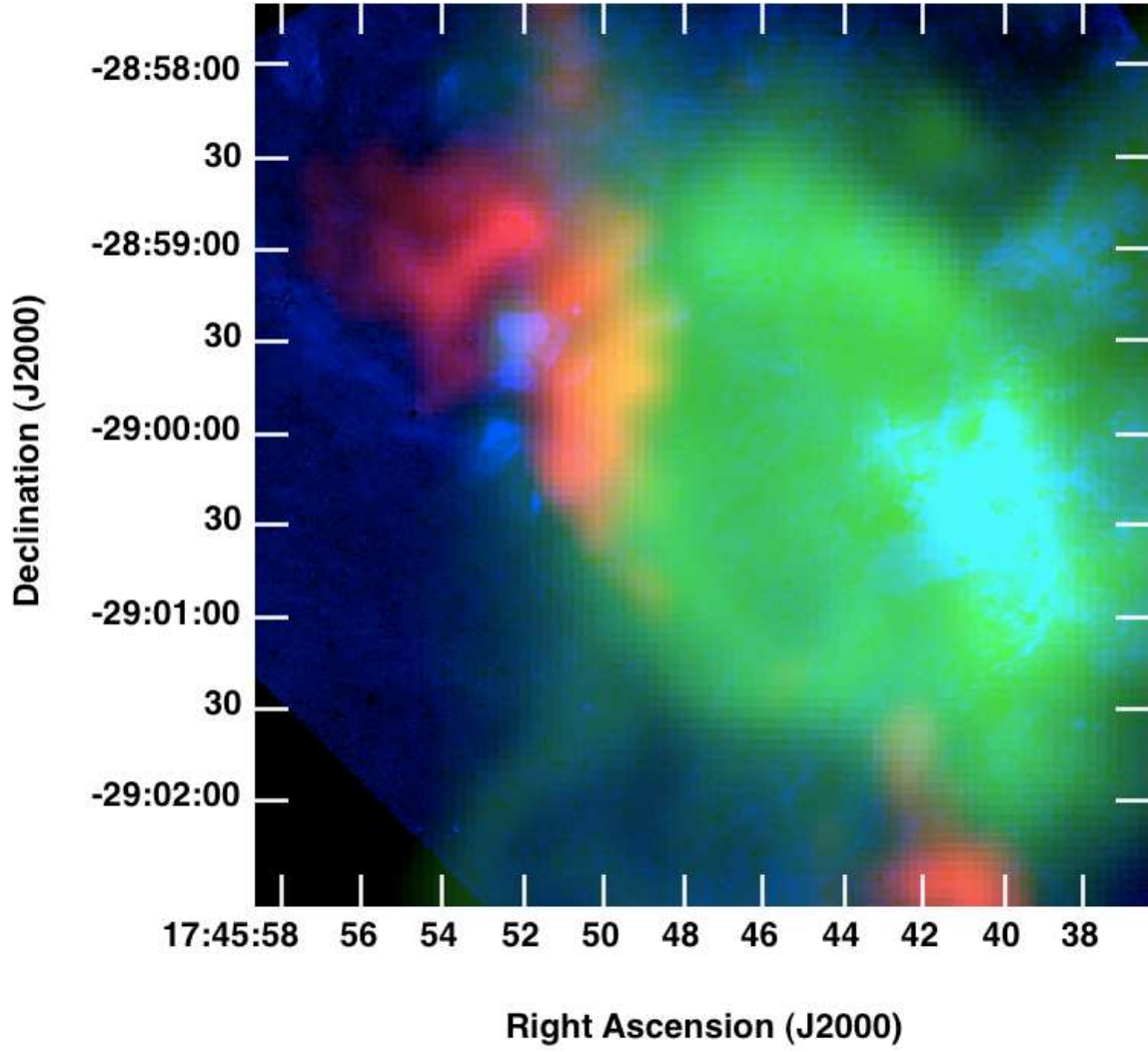
FIG. 3.— Composite image of P\alpha in blue, VLA 1.4 GHz data in green (Lang et al. 2010), and SCUBA 450 microns (Pierce-Price et al. 2000) in red. The main structures traced by P\alpha emission (blue) are the G-0.02-0.07 HII regions at middle left, and Sgr A West at lower right. The 1.4 GHz image (green) also traces these structures, but most prominent at 1.4 GHz is Sgr A East, the large shell of nonthermal emission that borders G-0.02-0.07 and appears to enclose Sgr A West. The 450 micron image (red) traces an entirely different component, the dense cool dust that corresponds to some of the densest parts of M-0.02-0.07, the 50 km/s molecular cloud, in which the HII regions appear embedded. At the bottom of the image, part of M-0.13-0.08, the 20 km/s cloud, can also be seen.
