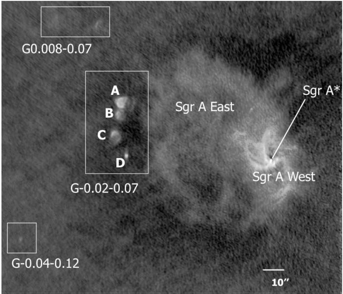
FIG. 1.— 8.4 GHz image showing the G-0.02-0.07 HII regions (A,B,C and D), the Sgr A East supernova remnant, and the Sgr A West complex of ionized gas surrounding the bright point source Sgr A*, the Galaxy’s central supermassive black hole. Also shown are two previously unknown radio sources, G0.008-0.07 and G-0.04-0.12. In this image, North is up, and East is to the Left.
