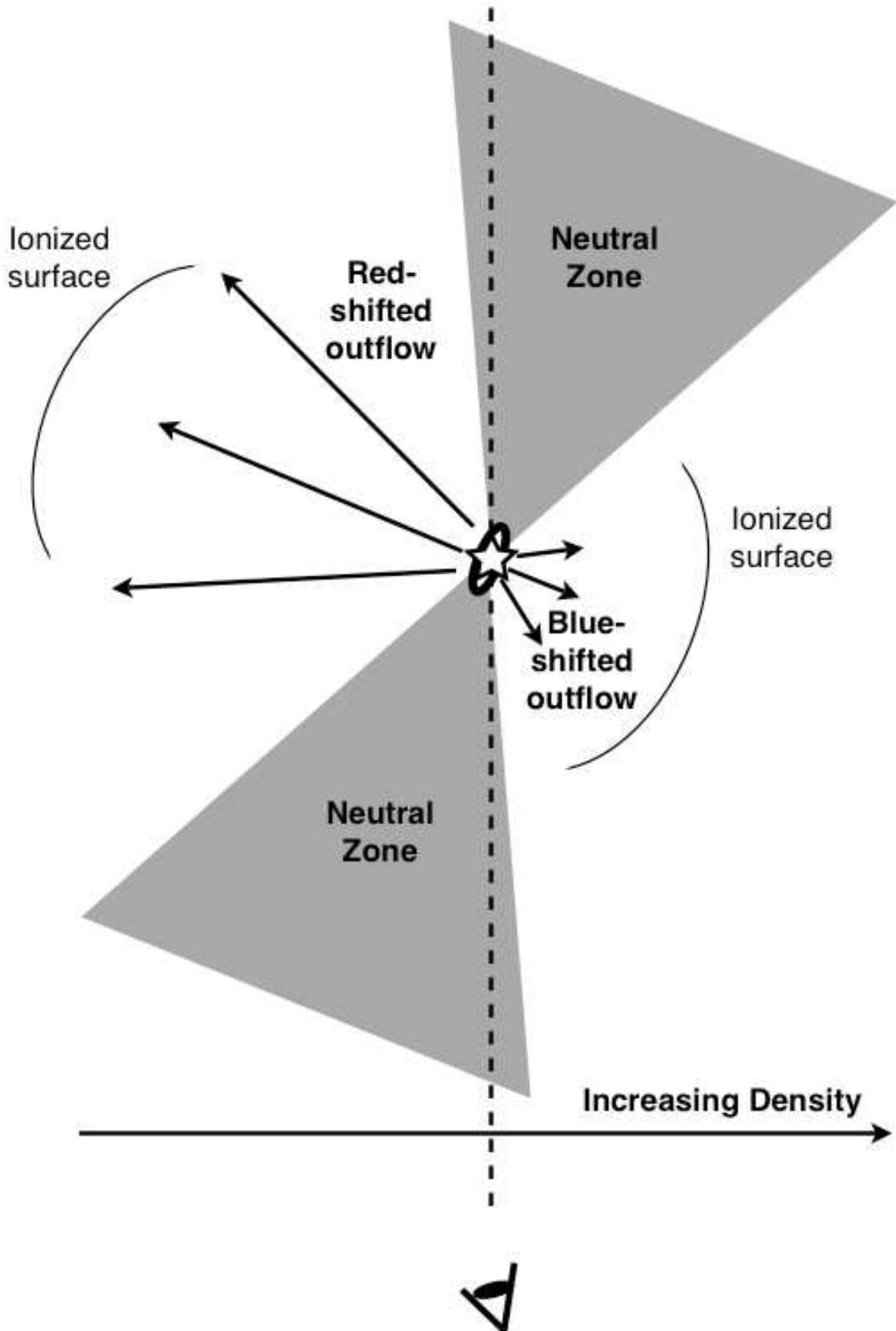
FIG. 8.— A model of the disk structure of region D. In this model, the disk at the center is small, and does not occult ionized emission along the line of sight, consistent with the lack of a high extinction value measured toward the location of the disk. We explain the dark lane visible in radio and P\alpha images which divides the two peaks of region D as due to disk absorption of ionizing radiation from the star. The dark lane represents a region of largely neutral gas which has been shielded from the ionizing radiation of the central star by the disk. The dominant source of the radio and P\alpha emission is the ionized surface of cavities evacuated by an outflow from the central disk. The edge of the western cavity appears to be located closer to the ionizing star, suggesting this cavity is smaller. This can be explained if region D is embedded in a density gradient which is increasing to the west.
