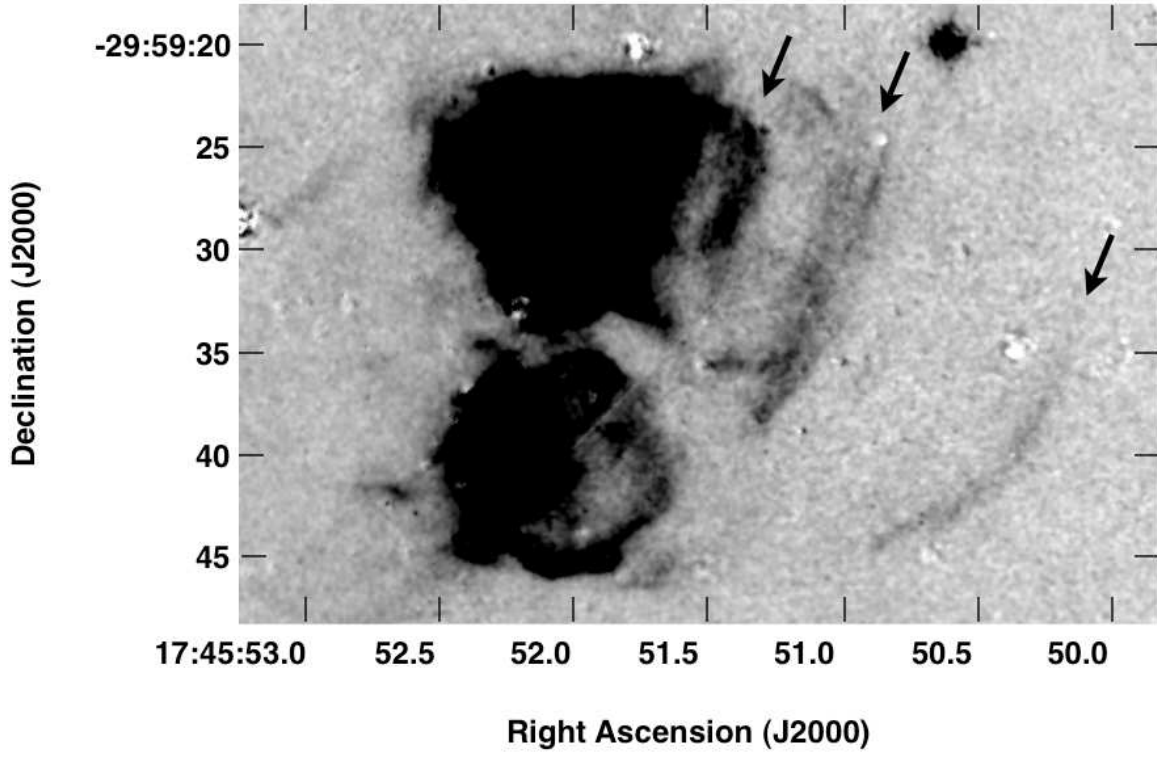
FIG. 11.— A magnification of the ionized ridges lying to the southwest of region A. The faint line that intersects region B at a 45 degree angle is an artifact from the edge of one of the mosaicked subimages used to construct this map.
