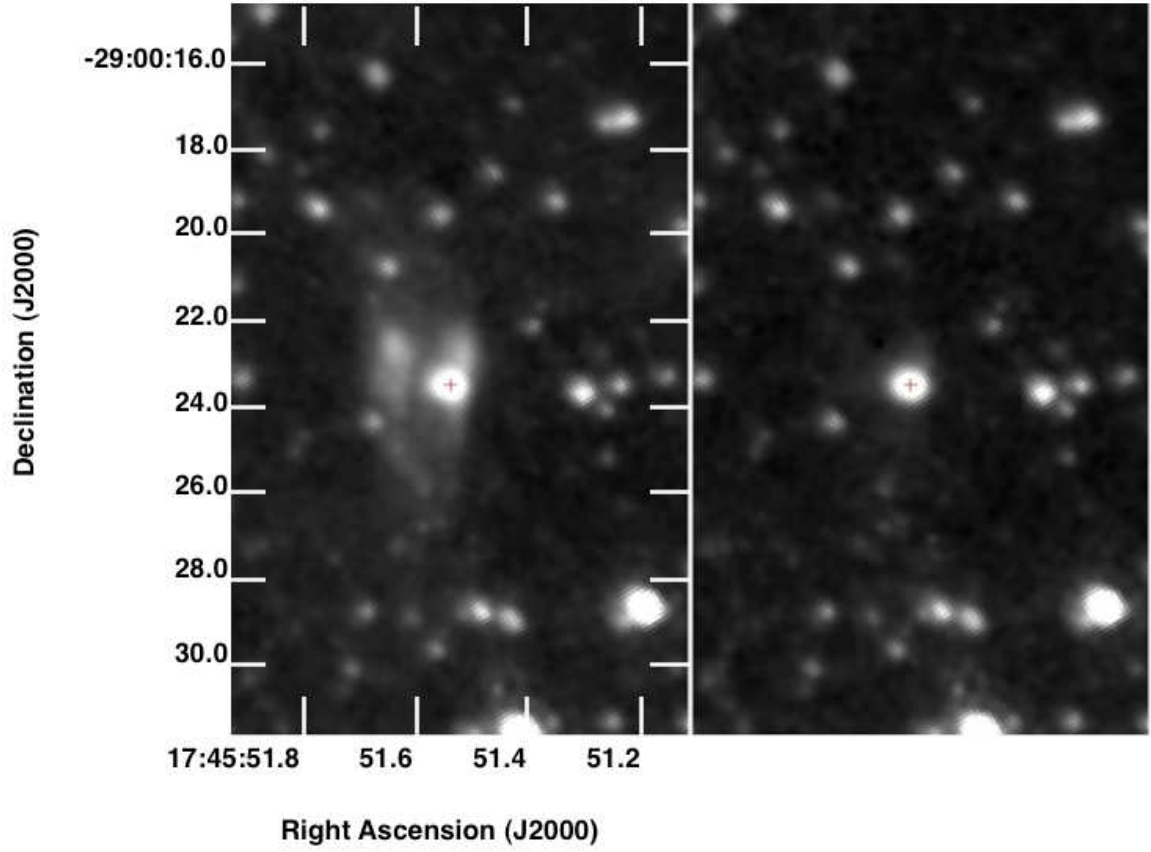
FIG. 7.— A comparison of the emission toward region D from the F187N and F190N filters. Slightly offset from the center of region D is a point source (indicated in both images with a cross) which has a F187N/F190N ratio consistent with being purely stellar continuum, with no excess emission from the P\alpha line. This point source was identified by Cotera et al. (1999) as having a stellar spectrum, and classified as a B[e] star (although this is not confirmed by our lack of detection of a P\alpha excess). They found the star to be highly reddened ( H-K' = 3.5 ), which corresponds to an extinction consistent with that which we measure toward region D, consistent with it being embedded in this region.
