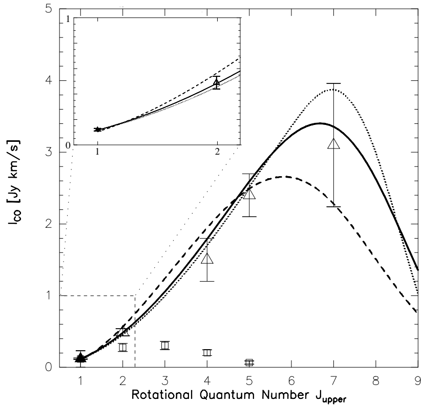
FIG. 4.— CO ladder and LVG models (based on all J > 1 transitions) for BR 1202-0725. The inset shows a zoomed-in version of the J = 2 , J = 1 region (as indicated by the dashed box). The filled triangle is the ^{12}\text{CO}(J=1\rightarrow 0) data point based on the combined spectrum. Data for the higher- J CO transitions (open triangles) are taken from the literature (see Table 3). For comparison, we also show data for the inner disk of the Milky Way (open squares, Fixsen et al. 1999), normalized to the ^{12}\text{CO}(J=1\rightarrow 0) flux of BR 1202-0725. The kinetic temperature T_{\text{kin}} and gas density \rho_{\text{gas}}(\text{H}_2) are treated as free parameters in this study. Three representative models are shown: Model 1 (solid line) assumes T_{\text{kin}} = 60 \text{ K} and \rho_{\text{gas}}(\text{H}_2) = 10^{4.1} \text{ cm}^{-3} , and gives the overall best fit to all transitions. Model 2 (dashed line) assumes T_{\text{kin}} = 120 \text{ K} and \rho_{\text{gas}}(\text{H}_2) = 10^{3.7} \text{ cm}^{-3} , while model 3 (dotted line) assumes T_{\text{kin}} = 30 \text{ K} and \rho_{\text{gas}}(\text{H}_2) = 10^{4.6} \text{ cm}^{-3} .
