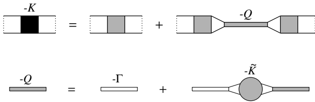
FIG. 2: Defining functions Q and \tilde{K} in the two-particle channel.
