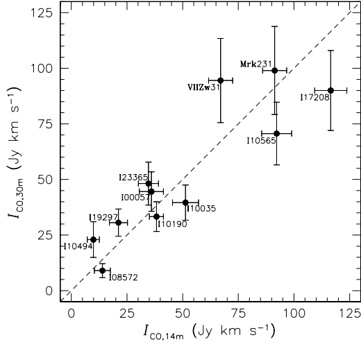
FIG. 5.— Comparisons of I_{CO} from the FCRAO 14m telescope with those measured by the IRAM 30m telescope (Solomon et al. 1997). The antenna gain, G=45 and 4.5 \text{ Jy K}^{-1} in T'_A and T_{mb} have been adopted for the 14m and 30m telescope, respectively. The 1-\sigma error bars are shown for both measurements. The dashed line shown is simply a linear relation that corresponds to I_{CO,30m} = I_{CO,14m} .
