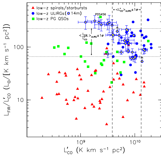
FIG. 9.— L_{FIR}/L'_{CO} vs. L'_{CO} . The same colored symbols are used as Figure 8. The dashed lines and the dotted lines represent L'_{CO} \pm 1\sigma ( 8.5 \pm 4.6 \times 10^9 \text{ K km s}^{-1} \text{ pc}^2 ) and L_{FIR}/L'_{CO} ( 145 \pm 79 L_\odot [\text{K km s}^{-1} \text{ pc}^2]^{-1} ) of 56 ULIRGs collected in this study. The error bars of our sample reflect the 1\sigma uncertainties in our CO measurements.
