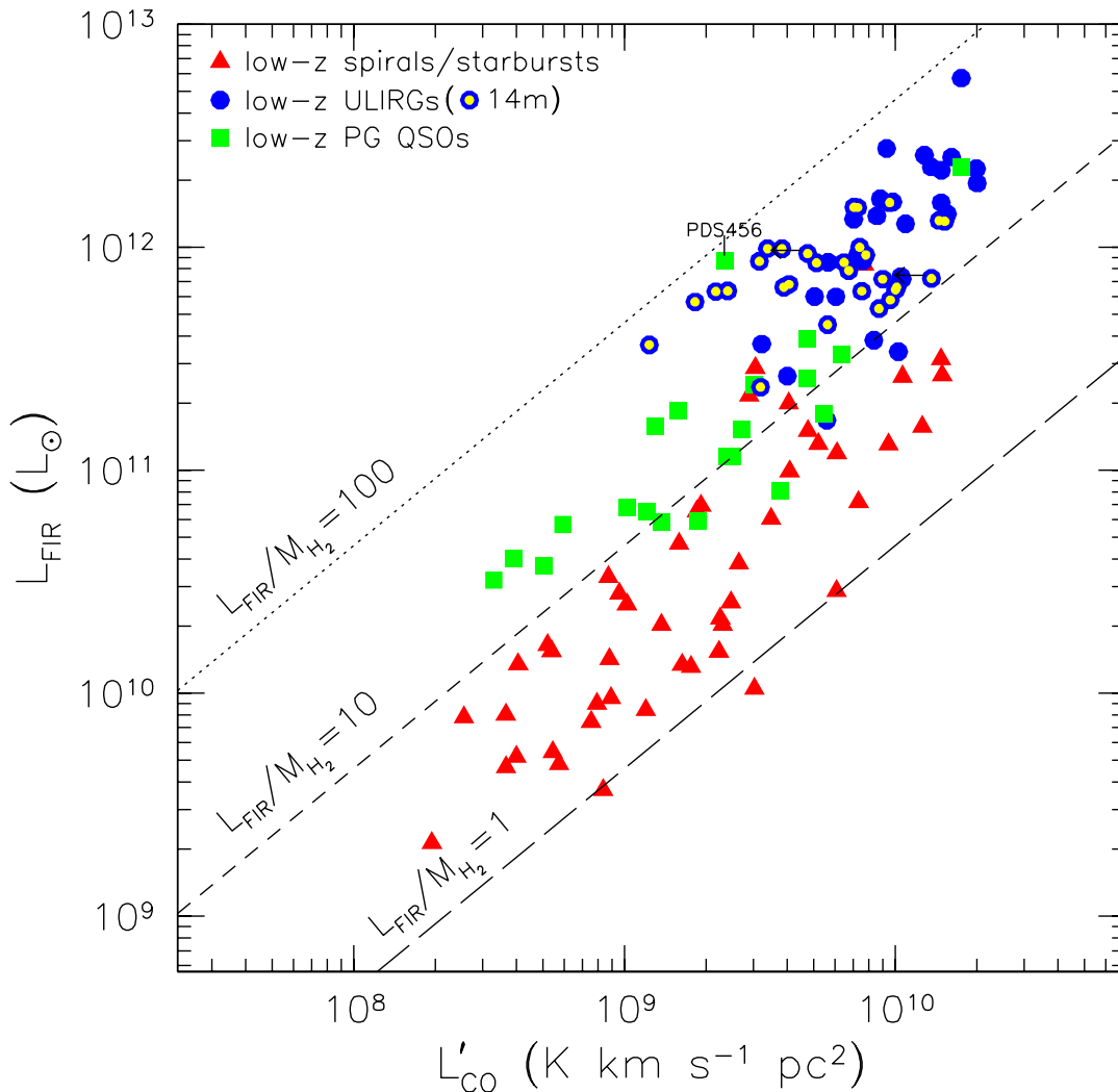
FIG. 8.— L_{FIR} vs. L'_{CO} of low- z galaxies with a range of far infrared luminosity. Spirals and starburst systems from Gao & Solomon (2004b) and Solomon et al. (1997) are shown red triangles, z \lesssim 0.3 Paloma- (PG) QSOs from Alloin et al. (1992), Evans et al. (2001), and Scoville et al. (2003) are shown by green squares. ULIRGs by Solomon et al. (1997) are shown in blue circles. The yellow dots with a blue circle around represent the ULIRGs in our sample observed by RSR on the FCRAO 14m telescope. Non-detections are indicated with arrows. Dotted and dashed lines indicate constant ratios of L_{FIR}/M_{H_2} = 1, 10, and 100 using the standard CO-to- H_2 conversion ( M_{H_2} [M_{\odot}] = 4.6L'_{CO} [K km s^{-1} pc^2] ).
