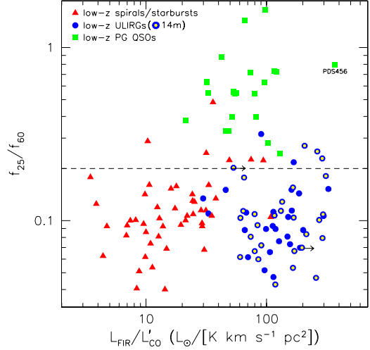
FIG. 10.— Infrared color ( f_{25}/f_{60} ) vs. L_{FIR}/L'_{CO} . The same colored symbols are used as as Figure 8. The dashed line represents f_{25}/f_{60} = 0.2 , the borderline of warm and cool ULIRGs.
