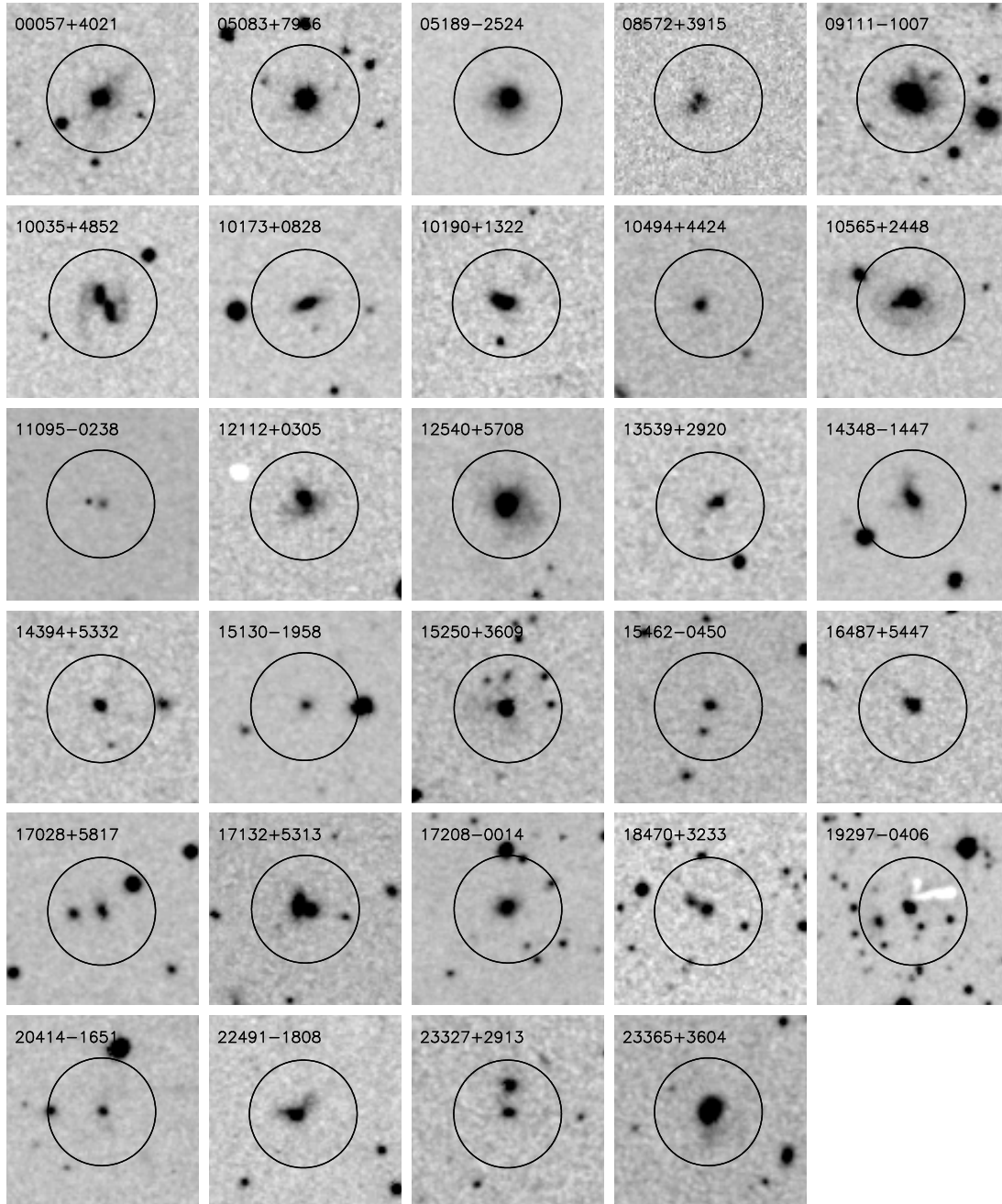
FIG. 1.— Optical images from the 2nd Digitized Sky Survey (DSS2) of the sample of 29 local ( z = 0.043-0.11 ) ULIRGs. Each field ( 1.5' \times 1.5' ) is centered on (\alpha, \delta)_{2000} as shown in Table 1. The IRAS catalog number is indicated on the top of each panel. A circle of 50'' ( \approx beamsize of 14m at 3mm) is shown in solid line.
