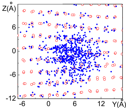
FIG. 3: (Color online) A columnar snapshot of atomic positions (open red dots) in the vicinity of the partial core (at the center) superimposed with the map (solid blue dots) of winding exchange cycles responsible for superfluid properties along the core, X -axis. Note that (i) the map extends over several unit cells ( \approx 3.67\text{\AA} ), and (ii) it has no visible structure in the Y -direction, implying negligibly small Peierls potential for climb at the simulated temperature.
