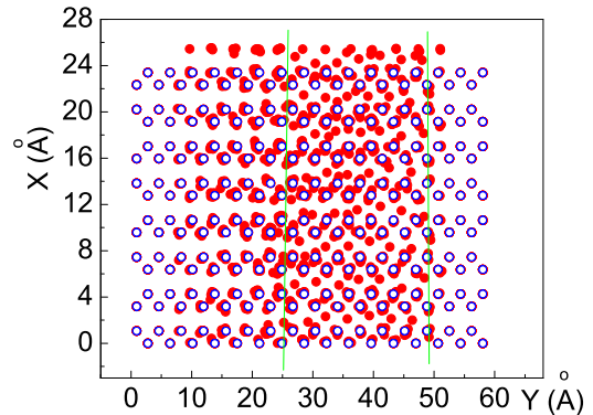
FIG. 1: (Color online) Columnar view of a typical MC configuration along the C-axis: filled red dots show atomic positions; open blue circles indicate an ideal lattice; vertical solid green lines mark positions of the partial cores. The fcc fault is between these two lines. The superfluidity occurs along the green lines.
