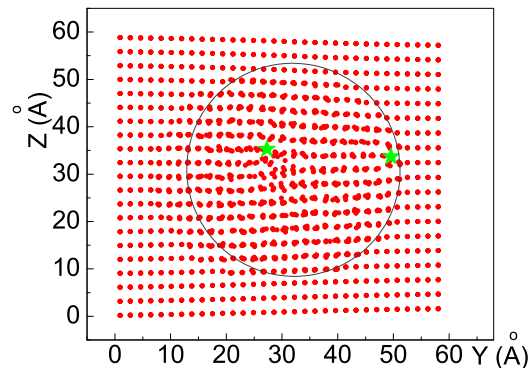
FIG. 2: (Color online) Columnar view of the same MC configuration (as in Fig. 1) along the cylinder axis. The circle marks the simulation cell where particle positions have been updated. The superclimb occurs in the “horizontal” plane. Green stars mark positions of the two partials.
