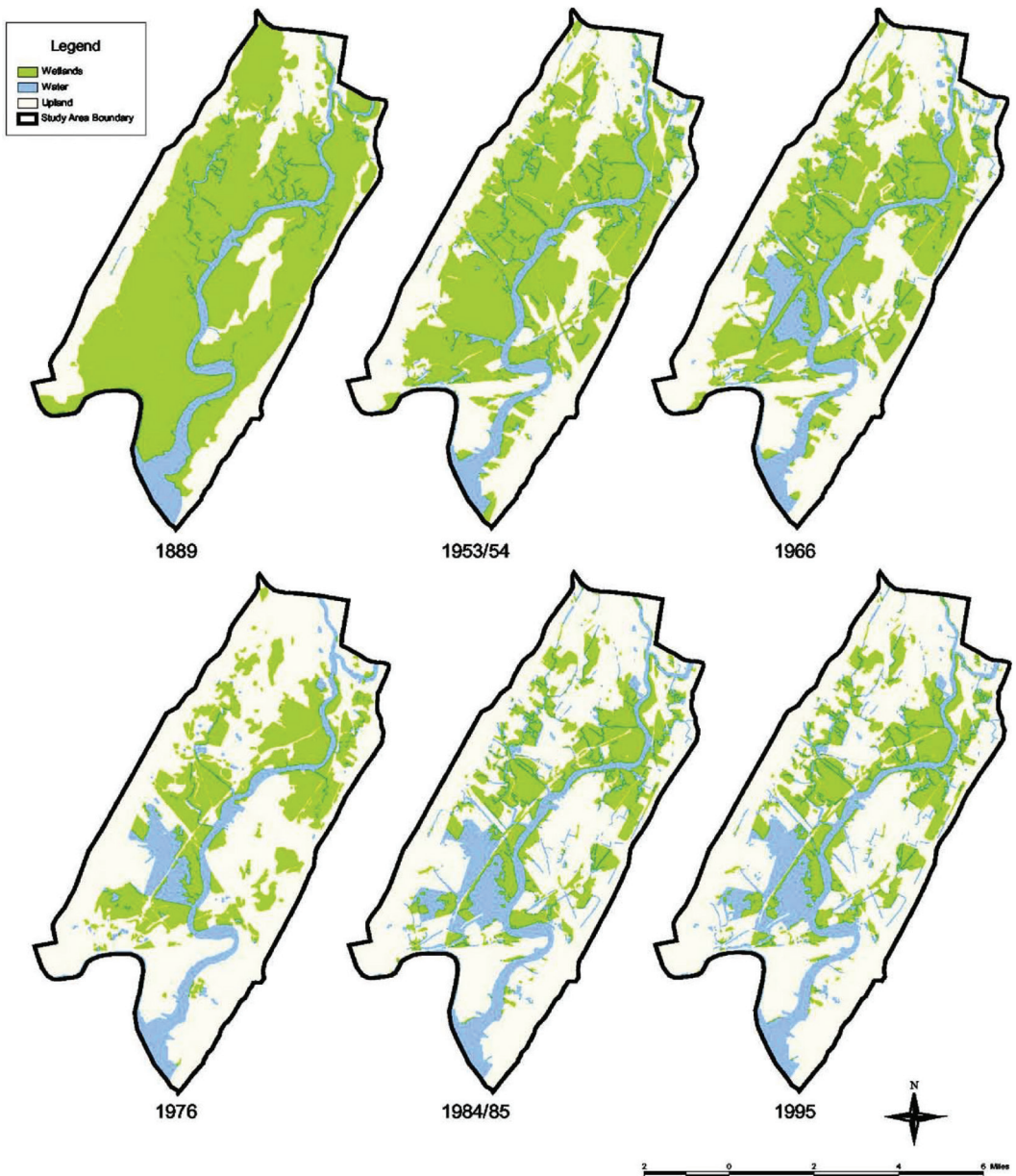
Figure 8.13. Changes in the Hackensack Meadowlands (NJ) from 1889 to 1995. While subjected to drainage, diking, and road construction since Colonial times, filling of the Meadowlands to create real estate accelerated after World War II. Wetland conversion slowed since the 1980s and today wetland restoration efforts are under way. (Tiner et al. 2002)
