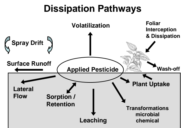
Illustration of the many processes associated with the breakdown of a pesticide courtesy http://www.epa.gov . Plant drawing courtesy http://aquat1.ifas.ufl.edu/drawlist.html
