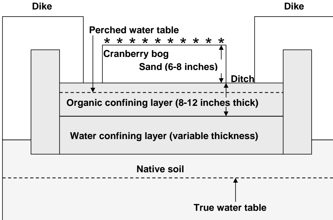
Cross-section of a cranberry bog constructed in mineral soil, not to scale. Organic and water confining layers create a perched water table. Diagram courtesy C. DeMoranville.
