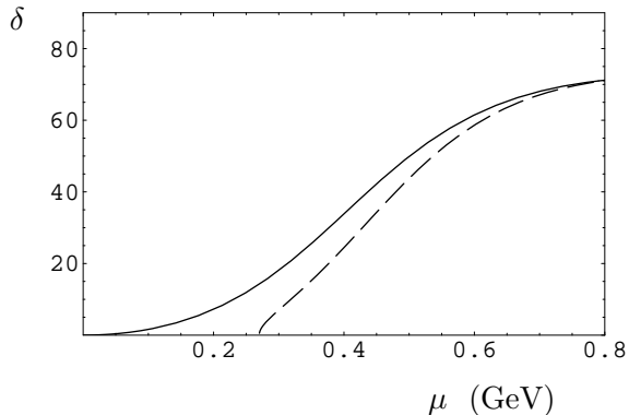
Figure 7: The scalar-isoscalar \pi\pi phase shifts using the IAM in the physical case (dashed line) and in the chiral limit (solid line).
