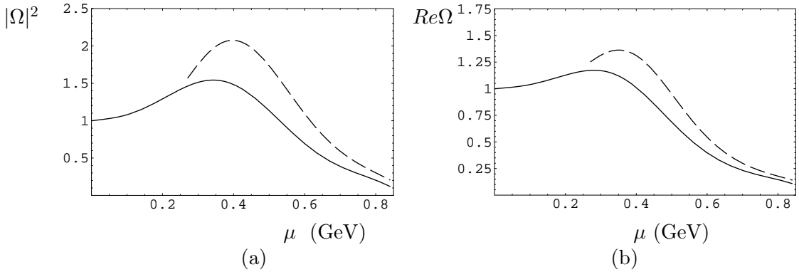
Figure 8: The absolute square (a) and the real part (b) of the Omnes functions in the physical case (dashed line) and in the chiral limit (solid line).
