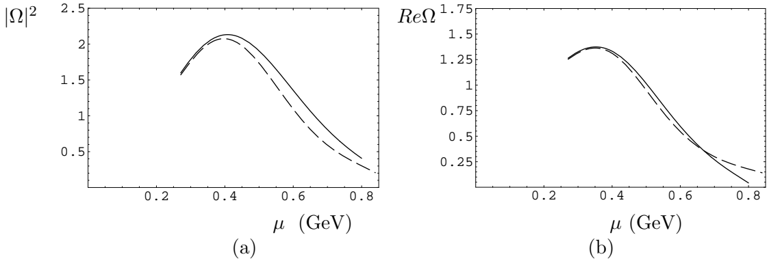
Figure 6: The absolute square (a) and the real part (b) of the Omnes functions derived from the CGL phase shifts (solid line) and those found using the inverse amplitude method (dashed line).
