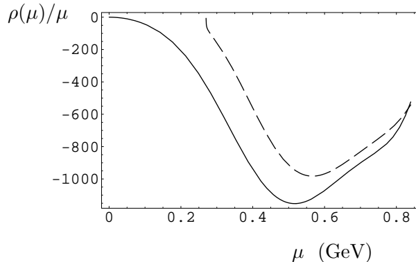
Figure 1: The spectral integrand, \rho_S(\mu)/\mu , whose integral determines the strength of the scalar-isoscalar interaction. The curve that extends down to \mu = 0 (solid line) is that for the chiral limit - the other (dashed line) is calculated with the physical pion mass.
