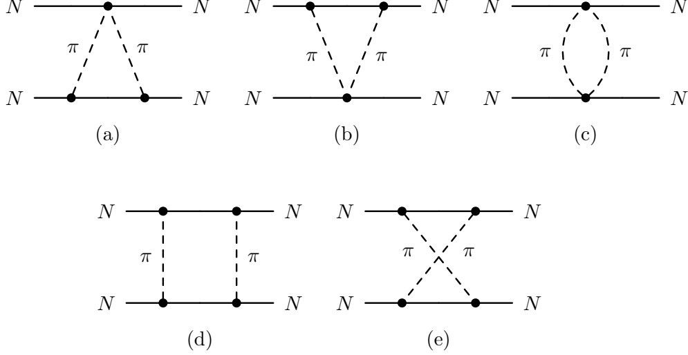
Figure 4: Two pion exchange diagrams which arise in chiral perturbation theory.
