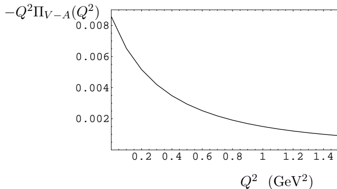
Figure 3: The figure shows the vacuum polarization function Q^2\Pi_{V-A}(Q^2) whose integral determines the chiral parameter g_{EM} . Notice that the greatest contribution comes from low energy.
