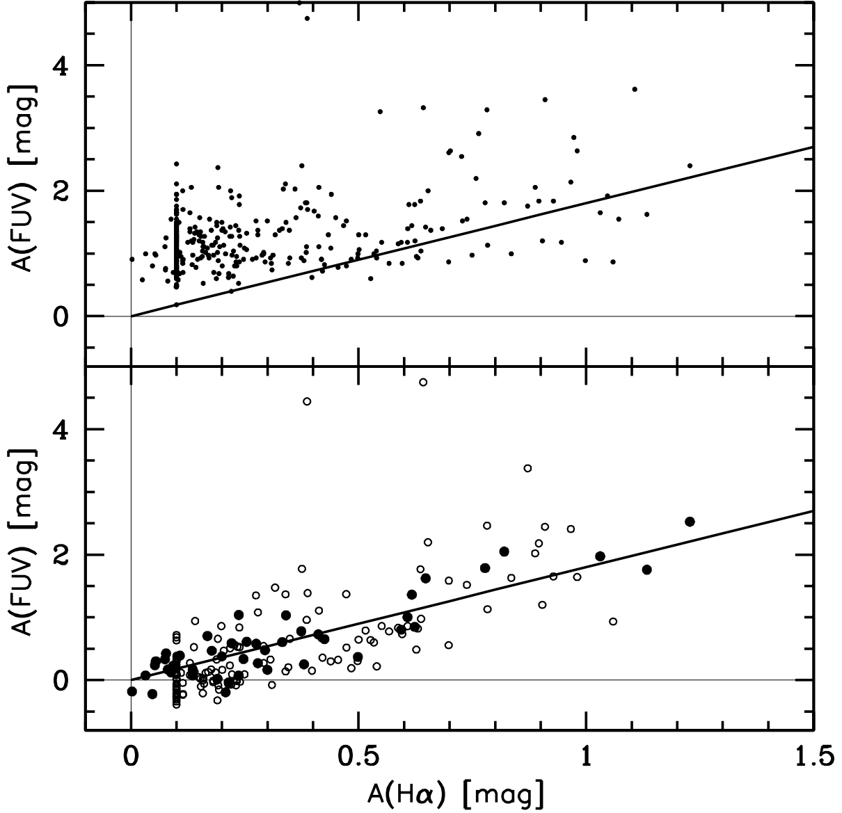
Fig. 4.— A comparison of different estimates of the H\alpha and FUV attenuation in galaxies in the 11HUGS sample. Bottom panel: FUV attenuations, A(\text{FUV}) , based on \text{TIR}/\text{FUV} ratios computed from MIPS photometry, and H\alpha attenuations A(H\alpha) based on (i) integrated spectroscopic measurements of the Balmer decrement (solid large points) and, (ii) A(H\alpha) estimated from a M_B dependent scaling relationship calibrated with Balmer decrement measurements (open points). Top panel: A(\text{FUV}) based on the linear \text{IRX}-\beta relationship of Cortese et al. (2006) and our best available value for A(H\alpha) (small black points). These latter A(\text{FUV}) estimates appear to be too high and are not used in our analysis. The solid line in both panels represents A(\text{FUV})=1.8A(H\alpha) , as expected for the Calzetti obscuration curve and differential extinction law. The Calzetti law provides a good description of our most robust attenuation measurements (solid large points).
