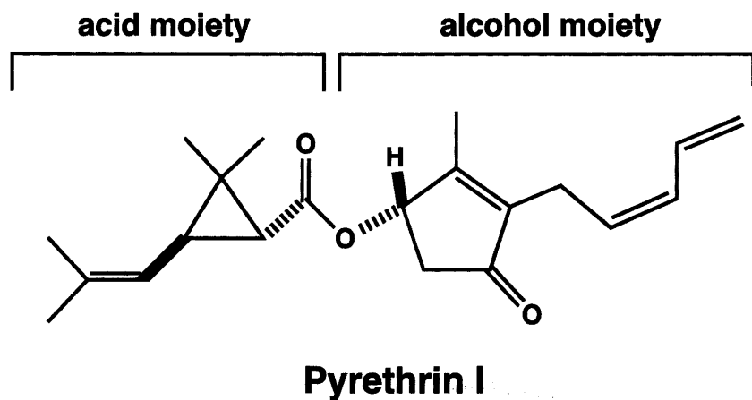
Figure 1. The chemical structure of pyrethrin I, the most toxic ester of pyrethrum. This structure is the basis for all pyrethroids (reproduced from Soderlund 2002).
