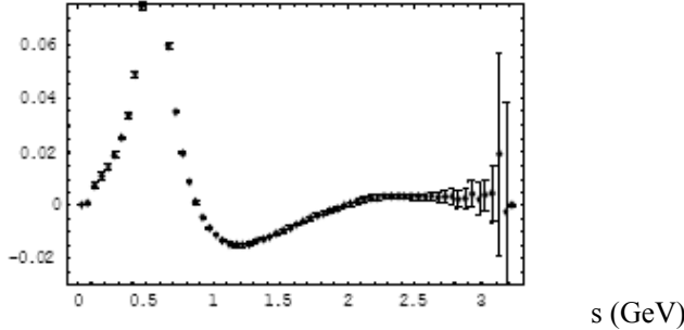
Fig. 1. The experimental spectral function \rho_{V-A}(s) which enters the dispersive predictions of the chiral parameters.
