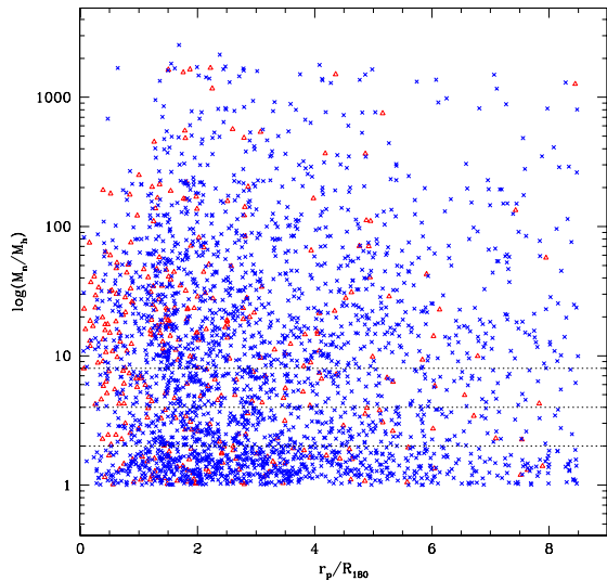
FIG. 5.— The nearest neighbor to host halo mass ratio M_n/M_h - projected distance r_p/R_{180} distribution of the dwarf central galaxies in samples S1+S2+S3. The triangles and crosses show the red and blue central galaxies, respectively, where the red population is defined to be the 20% reddest all galaxies.
