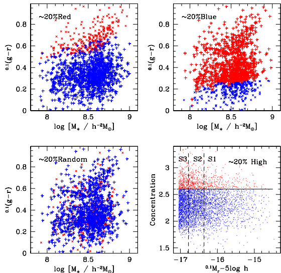
FIG. 3.— Upper-left panel: the color-stellar mass distribution of the 20% red (‘x’-crosses) and 80% blue (‘+’-crosses) dwarf galaxies in terms of similar stellar masses . Upper-right panel: the same set of dwarf galaxies as in the upper-left panel, but separated into 20% blue (‘x’-crosses) and 80% red (‘+’-crosses). Lower-left panel: the same set of dwarf galaxies as in the upper-left panel, but randomly selected and separated into 20% (‘x’-crosses) and 80% (‘+’-crosses) populations. Lower-right panel: the concentration-magnitude distribution of the dwarf galaxies, which are separated into \sim 20\% high and \sim 80\% low concentration populations by C = 2.6 .
