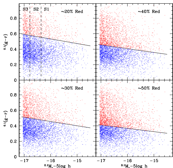
FIG. 1. — The color-magnitude distribution of dwarf galaxies (including central and satellite galaxies). In four panels the dwarf galaxies are separated into 20%, 30%, 40%, 50% red galaxies as indicated, respectively. The vertical dashed lines in the upper-left panel show the separation criteria of samples S1, S2 and S3.
