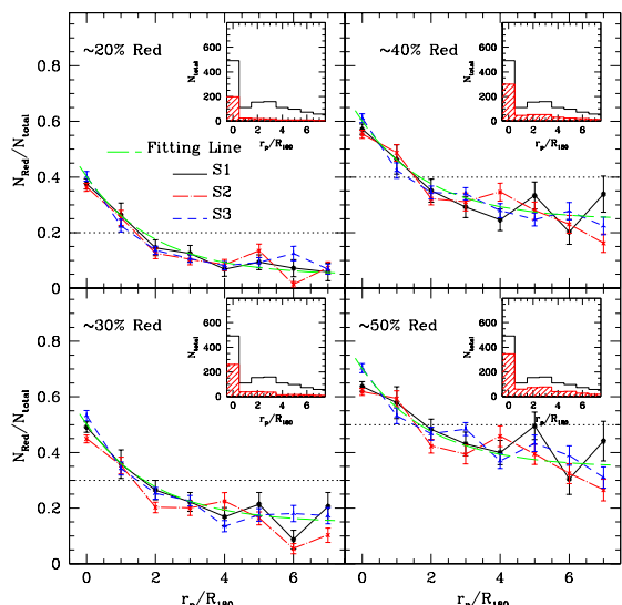
FIG. 2. — Fractions of the red central galaxies near more massive halos as a function of projected distance r_p/R_{180} . The four panels show the results of the color subsamples with 20%, 30%, 40% and 50% red galaxies, respectively. The related color subsample separation criteria are shown in Fig. 1. The different lines correspond to the different samples as indicated. The fit long-dashed, green line is described in the text. For comparison, we show the fraction of red satellite galaxies that are within the same luminosity ranges as the central galaxies at r_p/R_{180} = 0 . The small window within each panel shows the number counts of dwarf central (or satellite) galaxies in S1 as a function of r_p/R_{180} : black histogram for all galaxies and shaded, red histogram for red galaxies.
