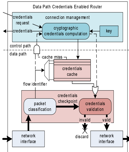
Figure 3.2. Router Architecture
