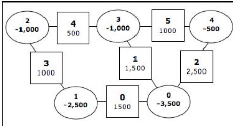
Figure 7. System Diagram Showing Line Limits and Loads
