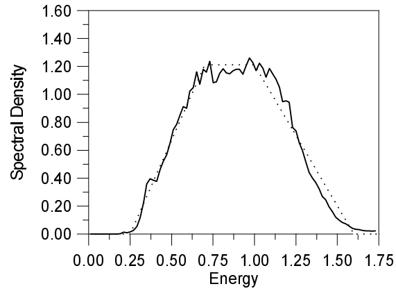
FIG. 17. The model spectrum (dashed lines) and results of spectral analysis (solid lines) for \eta = 10^{-2} (upper panel) and \eta = 10^{-3} (lower panel).
