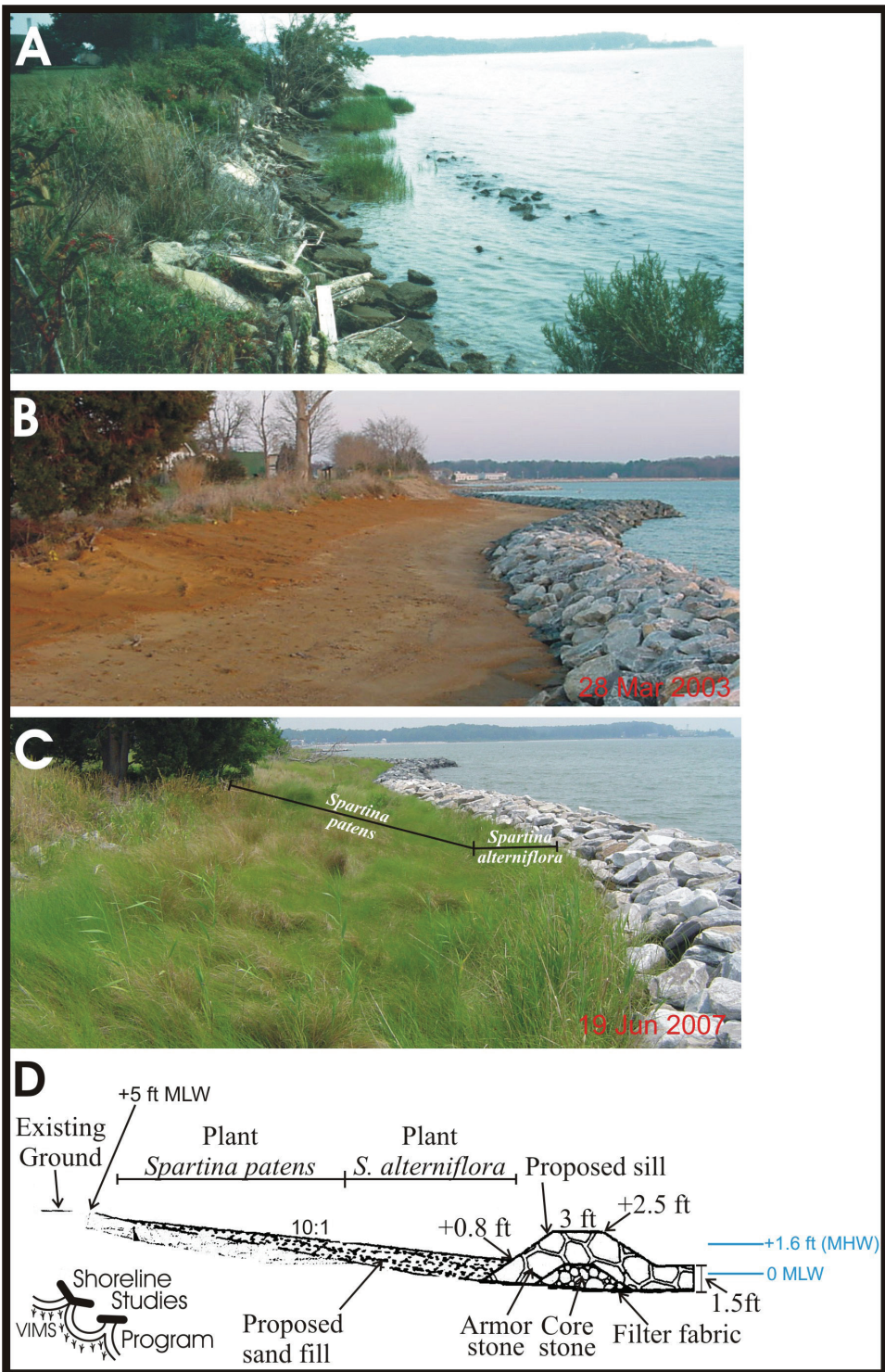
Figure 11.4. Living shorelines are a more natural solution to shoreline erosion that becomes part of the estuarine ecosystem as opposed to structural alternatives (e.g., bulkheads, seawalls, and rip-rap), which harden shorelines: (a) before; (b) during construction; (c) after construction; and (d) project plan. (Courtesy of Virginia Institute of Marine Science; Hardaway et al. 2009)
