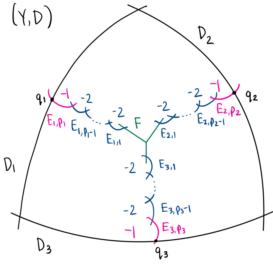
FIGURE 5.6. After (\bar{Y}, \bar{D}) is blown up arbitrarily many (p_i) times at each point q_i , the resulting pair is (Y, D) .
