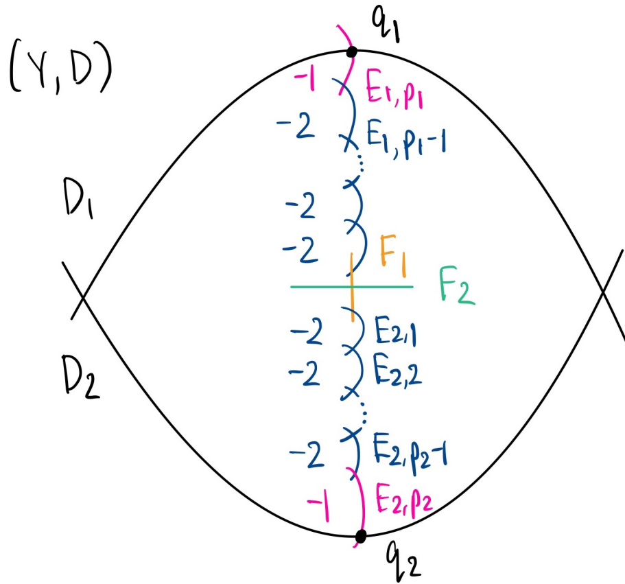
FIGURE 5.5. The blowup of (\bar{Y}, \bar{D}) at the two points q_1 and q_2 , a total of p_1 and p_2 times respectively, results in (Y, D) .
