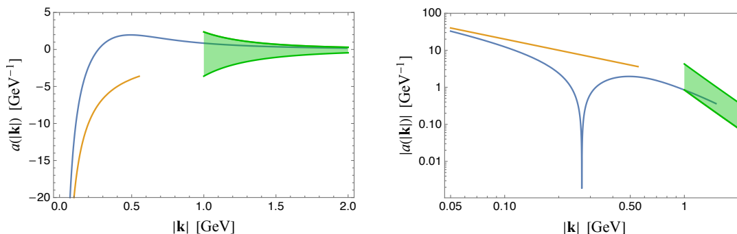
Figure 11. Left panel: a_{\chi}^{VV}(|\mathbf{k}|) (yellow), a_{<}^{VV}(|\mathbf{k}|, M_{\pi}) (blue), and a_{>}^{VV}(|\mathbf{k}|, M_{\pi}) (green) assuming \bar{g}_{LR}^{NN} \in [-10, 10] (lower to upper green curves and shaded band). Right panel: same plot for the absolute values in logarithmic scale.
