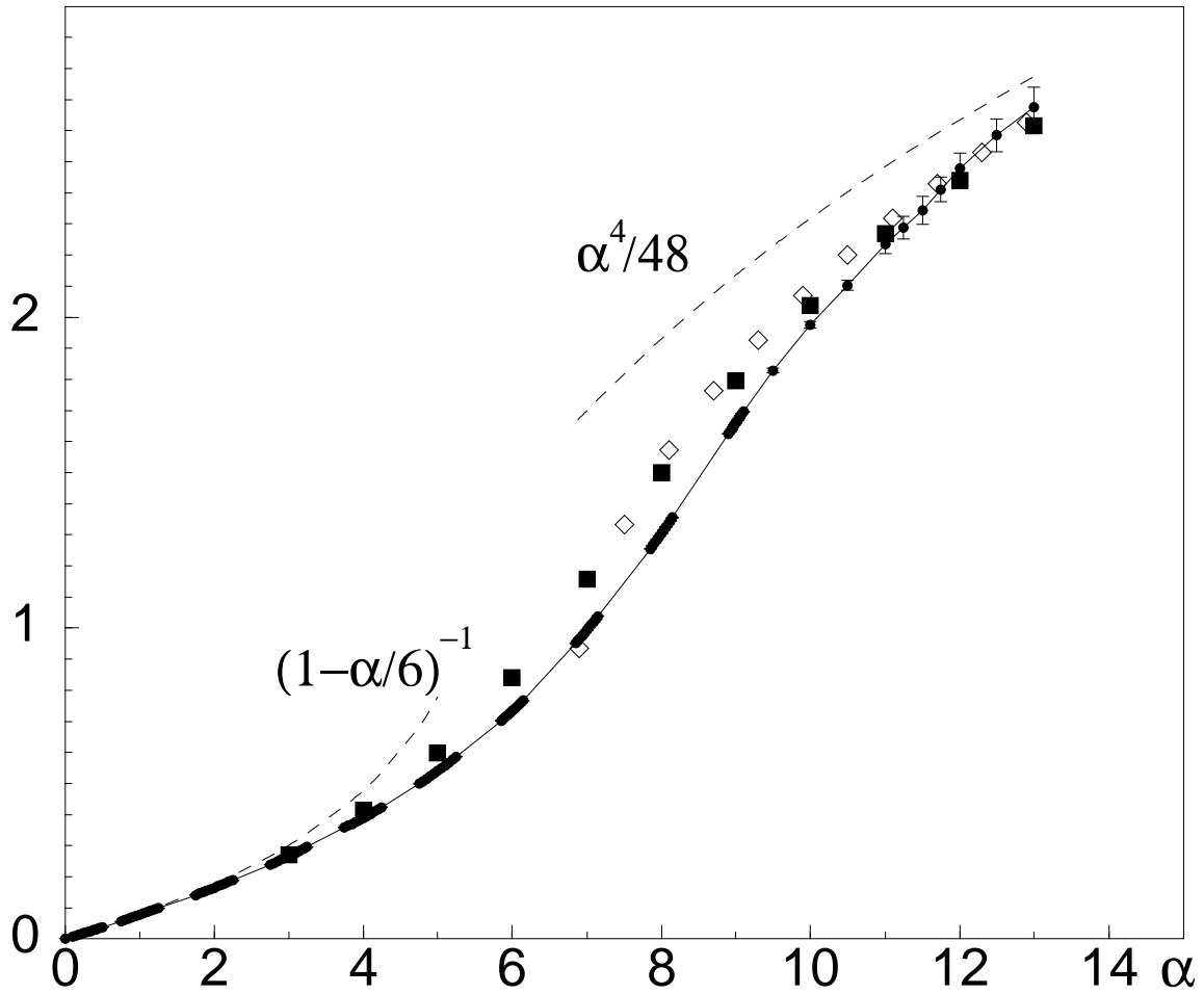
FIG. 5. Effective mass as a function of coupling parameter. Our MC data (circles interpolated by solid line) are compared with perturbation theory and strong-coupling-limit results (dashed lines), Feynman's approach (squares), and Feranchuk et. al. variational approach (diamonds).
