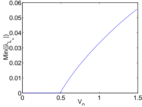
FIG. 9: The minimal-magnitude eigenvalue of L_+ as a function of V_0 for \phi_\star = 0 solutions. The 0 value of this diagnostic indicates the presence of modulational instability.
