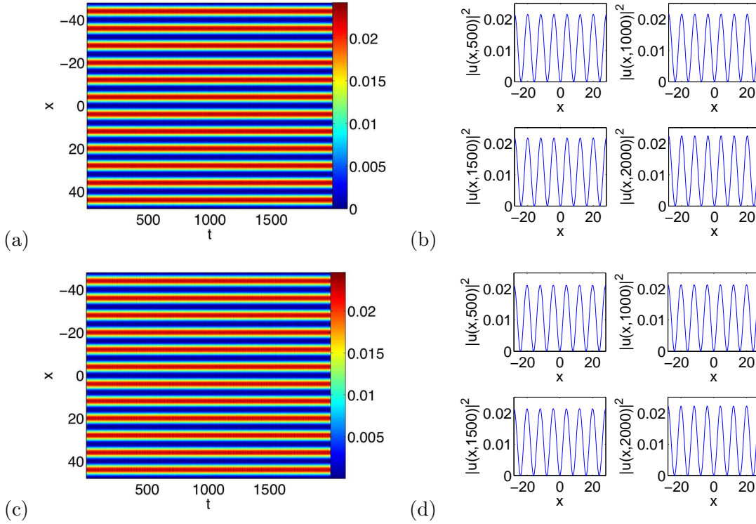
FIG. 6: (Color online) Dynamical evolution of the on-site solutions with \phi_* = \pi/2 for the initial waves of Eq. (23) [panels (a) and (b)] and Eq. (24) [panels (c) and (d)]. In both cases, V_0 = 0.15 .
