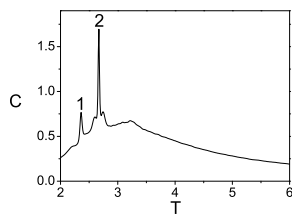
(g) 32^3 , \Delta_0 = 2.0 , seed: 1003
