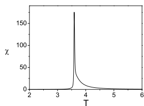
(f) 32^3 , \Delta_0 = 1.5 , seed: 1000
