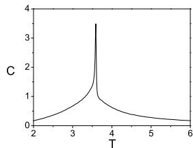
(e) 32^3 , \Delta_0 = 1.5 , seed: 1000
