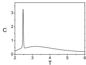
(c) 16^3 , \Delta_0 = 2.0 , seed: 1050
