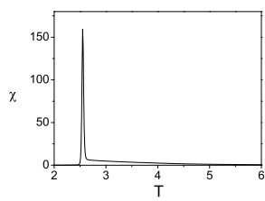
(b) 16^3 , \Delta_0 = 2.0 , seed: 1013
