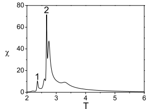
(h) 32^3 , \Delta_0 = 2.0 , seed: 1003
