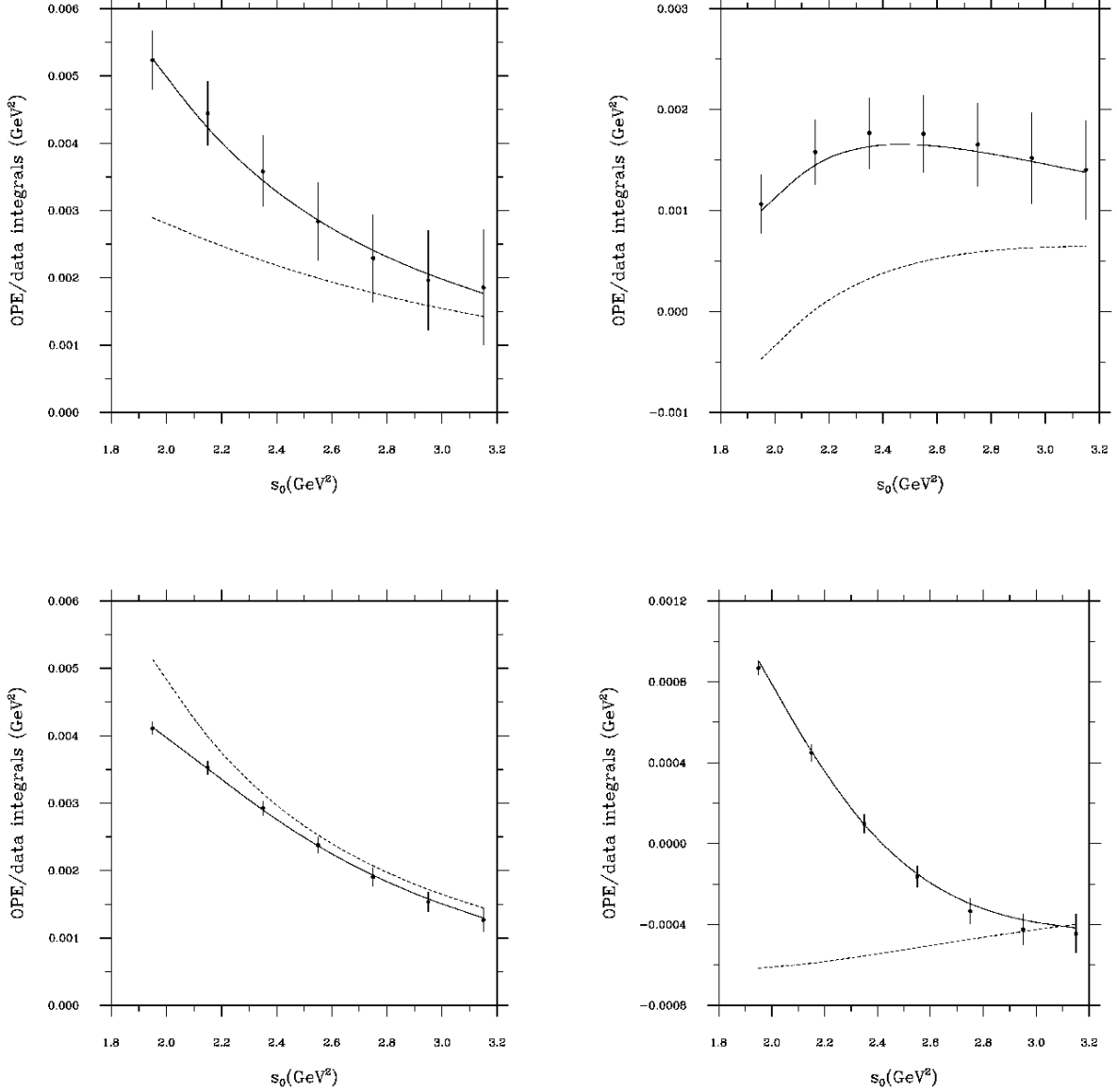
FIG. 6. J_{w(k,m)}(s_0) and f_{w(k,m)}(\{a_d\}; s_0) for the (0,0) (top left panel), (1,0) (top right panel), (1,1) (bottom left panel) and (1,2) (bottom right panel) spectral weight pFESR's. The J_{w(k,m)}(s_0) integrals and errors were obtained using the ALEPH data and covariance matrix. The dashed and solid curves correspond to the OPE fit of DGHS, and our combined fit (Eqs. (26)), respectively.
