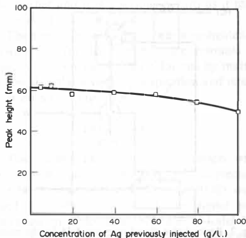
Fig. 4. Response of a constant concentration of copper as a function of the concentration of silver injected.
