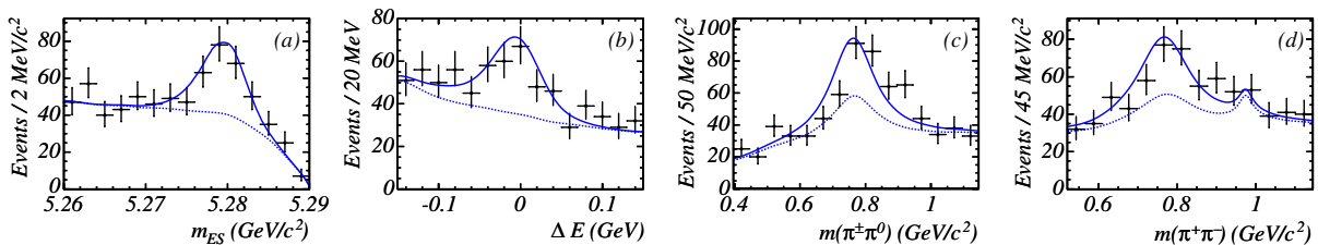
FIG. 1 (color online). Projections of (a) m_{ES} , (b) \Delta E , (c) m_{\pi^+ \pi^0} , and (d) m_{\pi^+ \pi^-} with a cut on the ratio of the signal and background likelihoods that selects about 40% of the signal. For (a) and (b), the observable plotted is excluded from the fit in calculating the likelihood used for the enrichment selection. For (c) and (d), only the m_{ES} , \Delta E , and x_{NN} variables have been used in calculating the likelihood. Points represent on-resonance data, dashed lines the continuum and B\bar{B} backgrounds PDFs, and solid lines the likelihood function with yields taken from the fit where all variables have been used.
