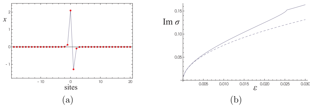
Figure 3. (a) The profile of an out of phase 2-site breather for \varepsilon = 0.02 . In (b) the imaginary part of \sigma_1 , for increasing values of \varepsilon , is shown. The solid line represents the numerically calculated value, while the dashed one is the one resulting from (14).
