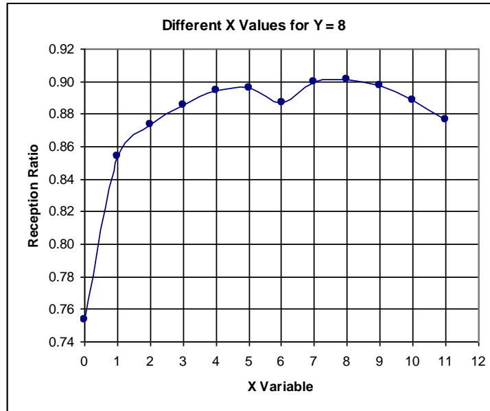
Figure 6.7 Reception ratio vs. X for UGS in Highway Simulations
