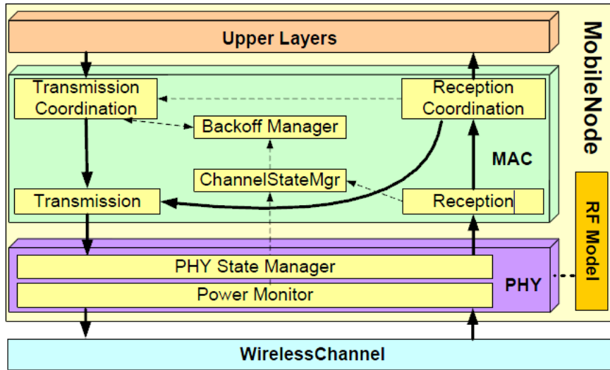
Fig. 4.1 Revised IEEE 802.11 Simulation Architecture [26]
