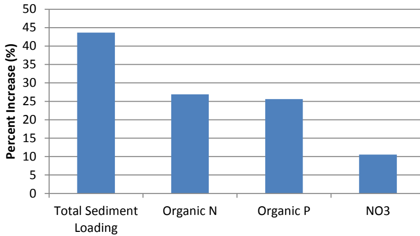
Figure 3.3 Percent increase in average annual water quality parameters (total sediment loading, organic N and P, nitrate [NO 3 ])
