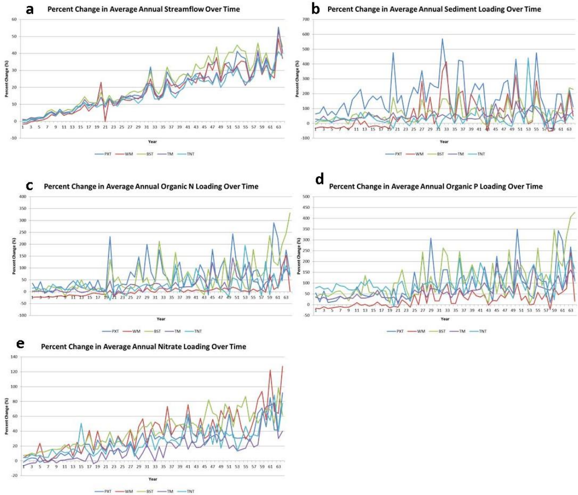
Figure 5.2 Percent change relative to baseline over time in annual averages for streamflow (a), total sediment loading (b), organic N loading (c), organic P loading (d) and nitrate loading (e). PXT=Pawtuxet, WM= Woonasquatucket-Moshassuck, BST= Blackstone, TM=Ten Mile, TNT=Taunton.
