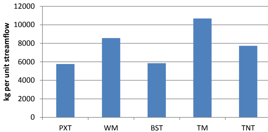
Figure 2.7 Normalized average annual loading of sediment, organic nitrogen (N) and organic phosphorus (P). PXT=Pawtuxet, WM= Woonasquatucket-Moshassuck, BST= Blackstone, TM=Ten Mile, TNT=Taunton.
