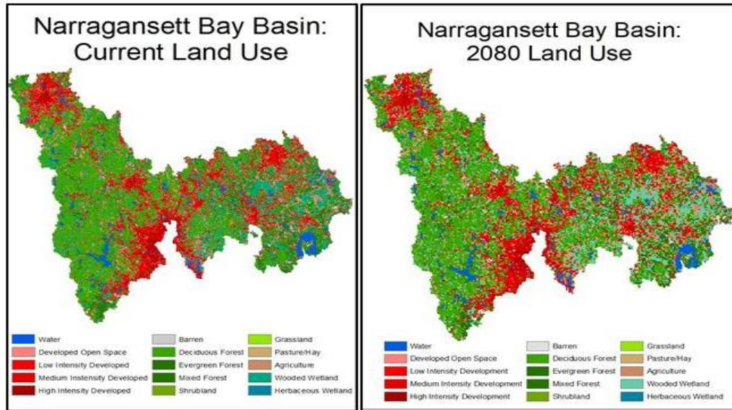
Figure 4.1 Land cover in the Narragansett Bay Basin at current (left) and projected 2080 (right).
