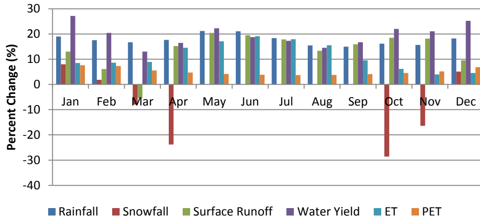
Figure 3.2 Percent change in average monthly hydrological parameters
