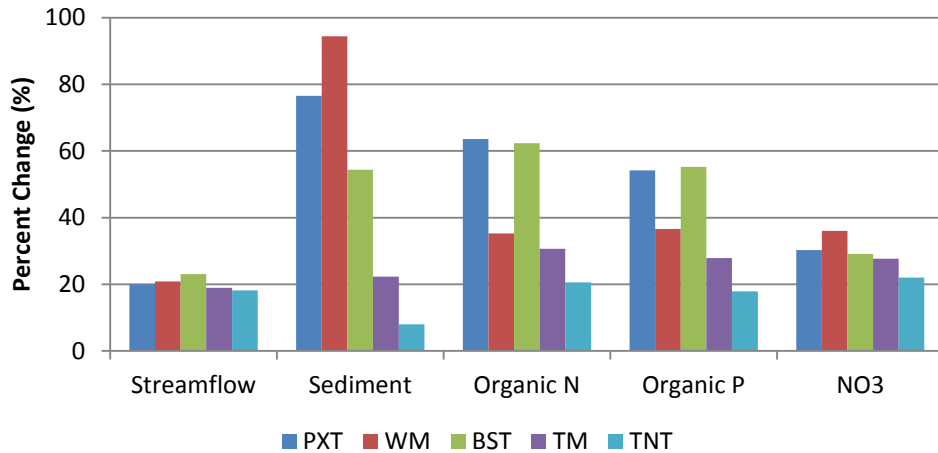
Figure 3.4 Percent change in average annual streamflow and water quality parameters (PXT=Pawtuxet, WM= Woonasquatucket-Moshassuck, BST= Blackstone, TM=Ten Mile, TNT=Taunton).
