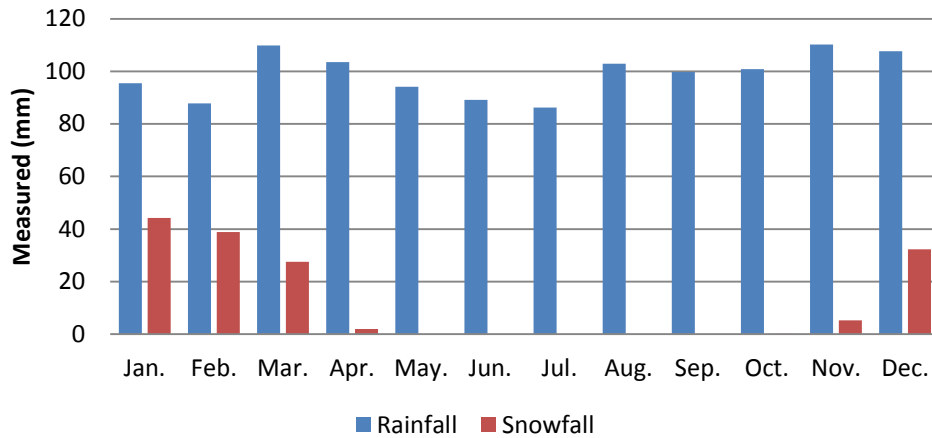
Figure 2.1 Average monthly precipitation in the Narragansett Bay Basin under baseline conditions
