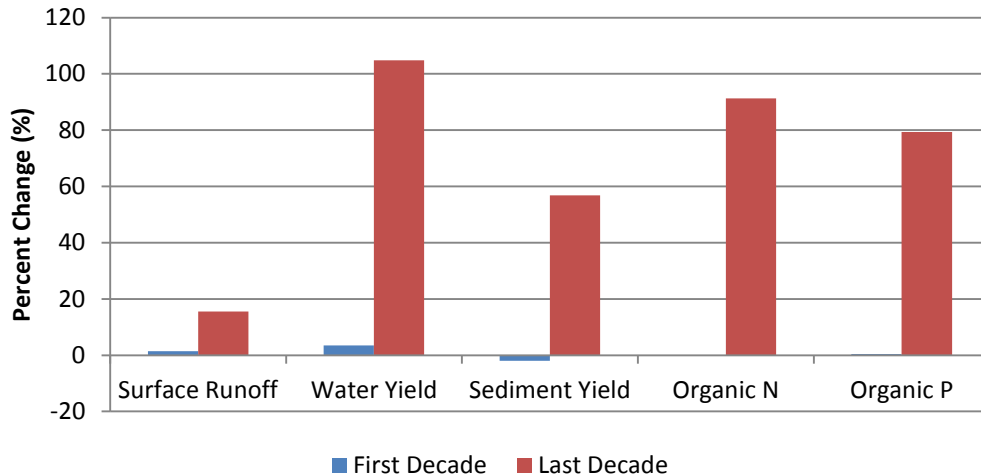
Figure 3.3 Percent change in water quantity and quality parameters in the first and last decade of the simulation.
