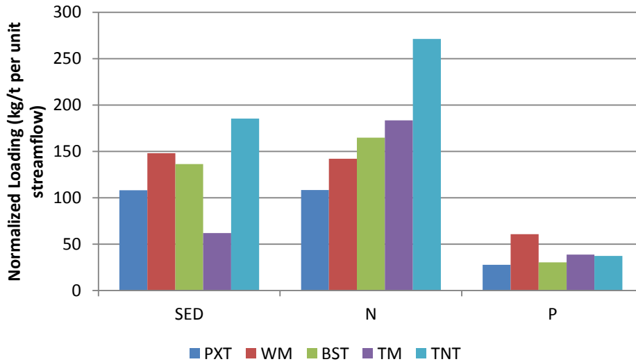
Figure 2.7 Normalized average annual loading of sediment, organic nitrogen (N) and organic phosphorus (P). PXT=Pawtuxet, WM= Woonasquatucket-Moshassuck, BST= Blackstone, TM=Ten Mile, TNT=Taunton.
