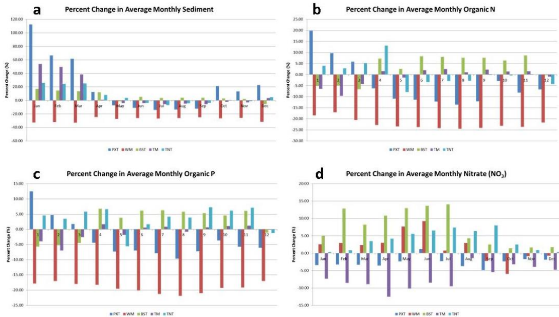
Figure 4.3 Percent change in monthly averages for total sediment loading (a), organic N loading (b), organic P loading (c) and nitrate loading (d). PXT=Pawtuxet, WM=Woonasquatucket-Moshassuck, BST= Blackstone, TM=Ten Mile, TNT=Taunton.
