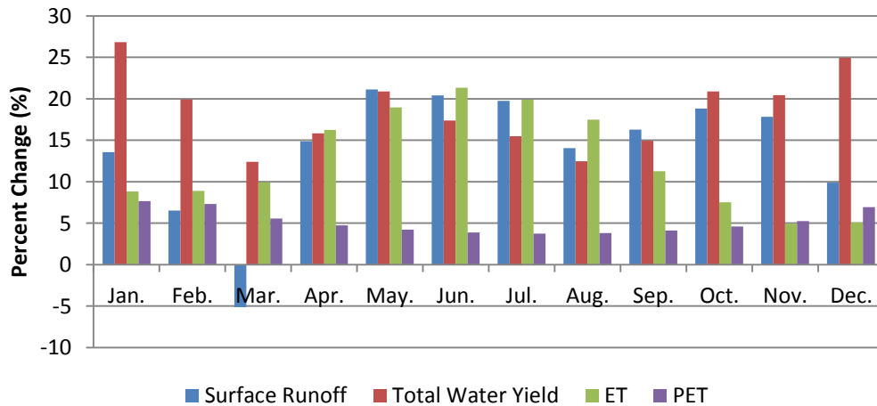
Figure 5.1 Percent change in average monthly values relative to baseline simulation.
