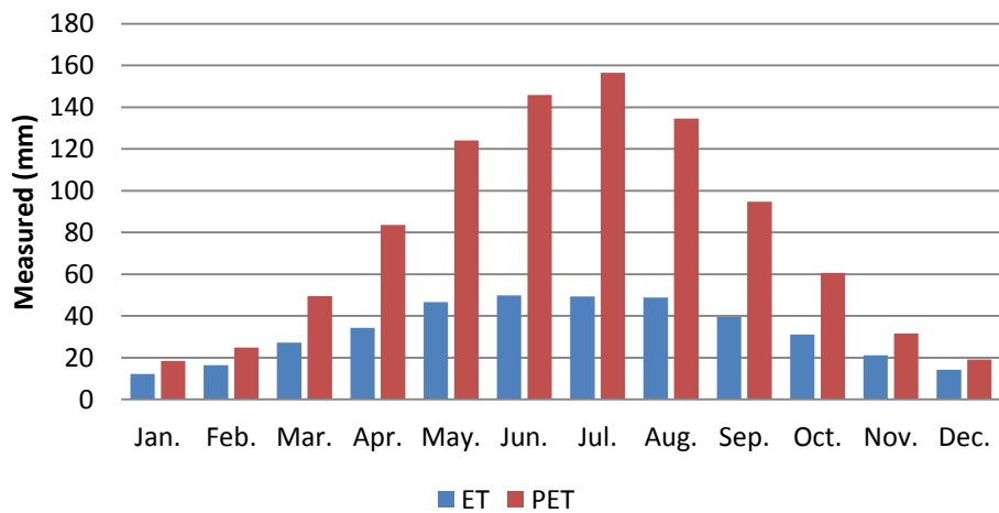
Figure 1.4 Average monthly evapotranspiration (ET) and potential evapotranspiration (PET) in the Narragansett Bay Basin
