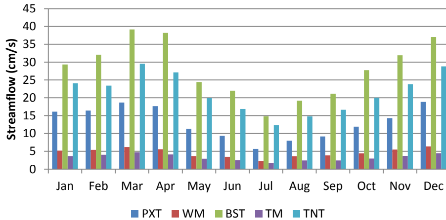
Figure 2.6 Average monthly streamflow for the five major rivers in the Narragansett Bay Basin (PXT=Pawtuxet, WM= Woonasquatucket-Moshassuck, BST= Blackstone, TM=Ten Mile, TNT=Taunton)
