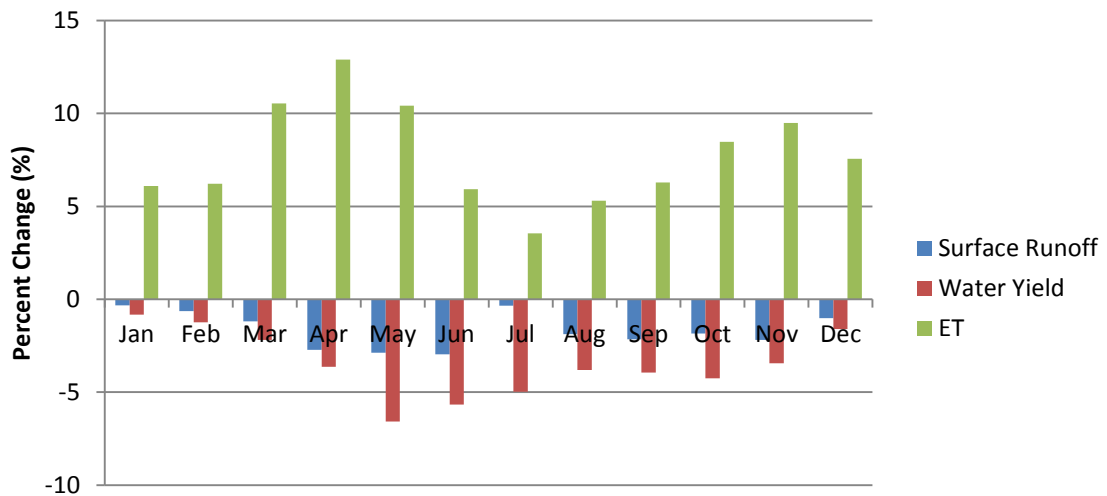
Figure 4.2 Percent change in average monthly values for Narragansett Bay Basin
