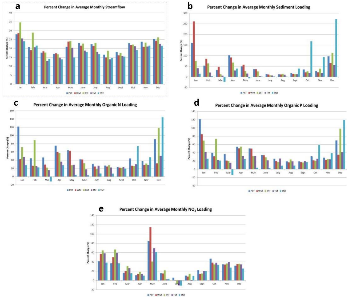
Figure 3.5 Percent change in monthly averages for streamflow (a), total sediment loading (b), organic N loading (c), organic P loading (d) and nitrate loading (e). PXT=Pawtuxet, WM=Woonasquatucket-Moshassuck, BST= Blackstone, TM=Ten Mile, TNT=Taunton.
