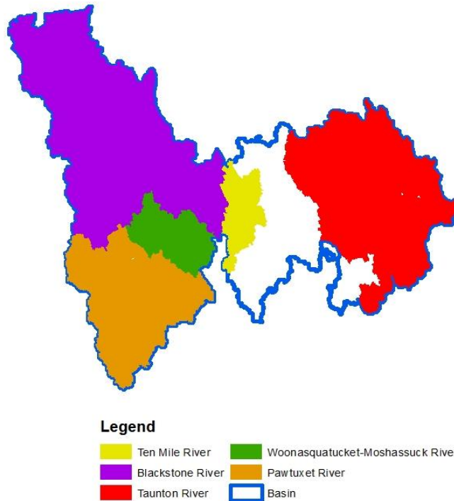
Figure 2.5 Five major watersheds studied: Ten Mile, Blackstone, Taunton, Woonasquatucket-Moshassuck and Pawtuxet Rivers
