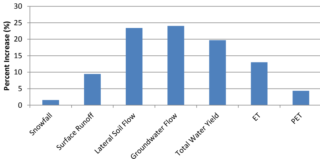
Figure 2.1 Percent increase in average annual hydrological parameters
