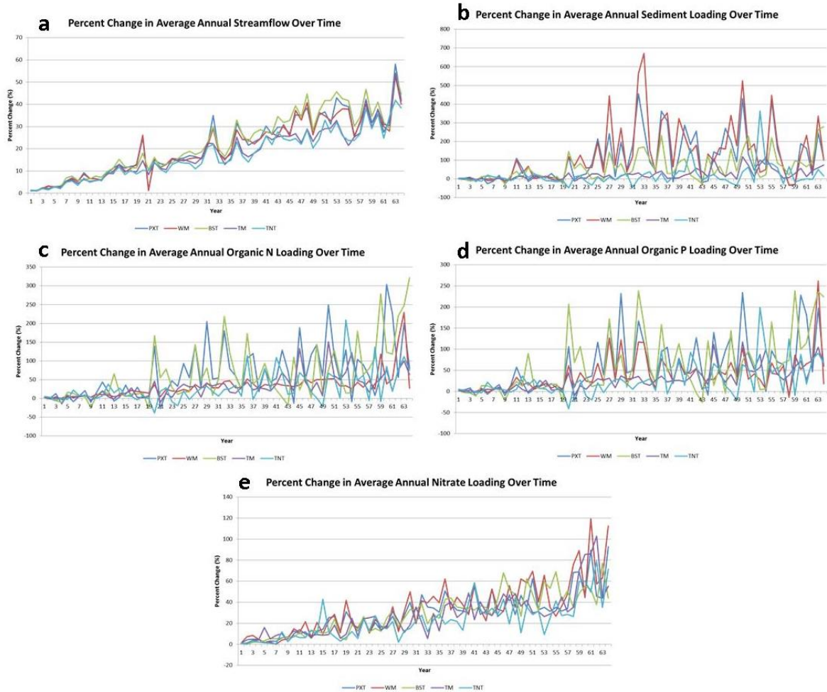
Figure 3.6 Percent change over time in annual averages for streamflow (a), total sediment loading (b), organic N loading (c), organic P loading (d) and nitrate loading (e). PXT=Pawtuxet, WM= Woonasquatucket-Moshassuck, BST= Blackstone, TM=Ten Mile, TNT=Taunton.
