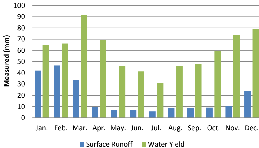
Figure 2.3 Average monthly surface runoff and total water yield in the Narragansett Bay Basin
