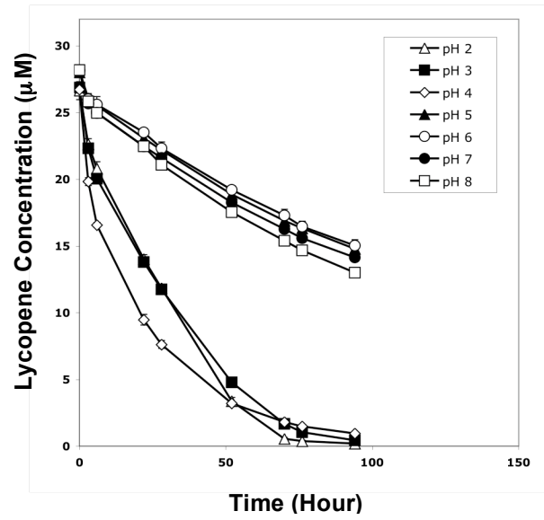
Figure 4.3: Lycopene concentration over storage time in SDS-stabilized emulsions at pH 2-8 stored at 15°C. Data points represent means (n=3) \pm standard deviations. Some error bars lie within the data points.
