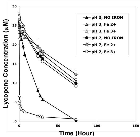
Figure 4.5: Lycopene concentration over storage time at room temperature in SDS-stabilized emulsions at pH 3.0 or 7.0, with 100 \mu\text{M} ferrous iron, 100 \mu\text{M} ferric iron, or no iron added. Data points represent means ( n=3 ) \pm standard deviations. Some error bars lie within the data points.
