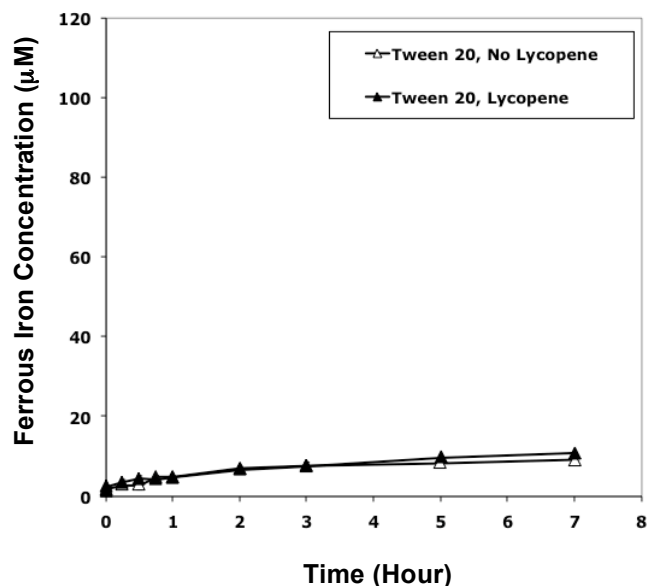
Figure 5.6: Ferrous iron concentration over time in Tween 20-stabilized emulsions with and without lycopene after the addition of (A) 100 µM ferrous sulfate, or (B) 100 µM ferric chloride. Data points represent means ( n=2 ) \pm standard deviations. Some error bars lie within the data points.
