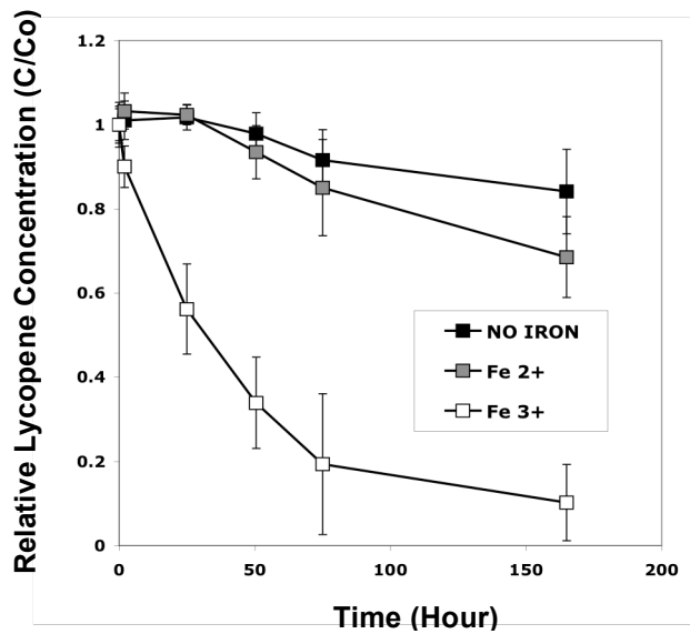
Figure 4.6: Lycopene concentration over storage time at room temperature in hexadecane with 11 uM lycopene and 100 uM ferrous iron, 100 uM ferric iron, or no iron added. Data points represent means (n=3) \pm standard deviations. Some error bars lie within the data points.
