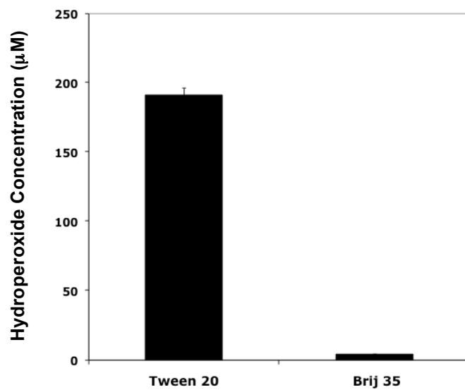
Figure 5.4: Hydroperoxide concentration of 30 mM Tween 20 and Brij 35 solutions. Data points represent means (n=6) \pm standard deviations.
