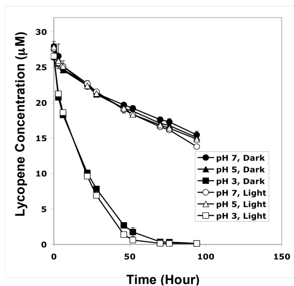
Figure 4.1: Lycopene concentration over storage time in SDS-stabilized emulsions at pH 3.0, 5.0, or 7.0 stored in light or dark conditions at 15°C. Data points represent means (n=3) \pm standard deviations. Some error bars lie within the data points.
