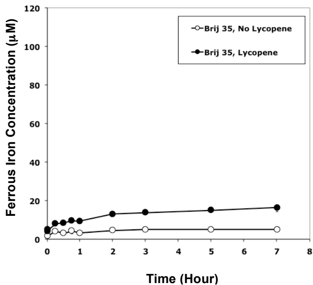
Figure 5.7: Ferrrous iron concentration over time in Brij 35-stabilized emulsions with and without lycopene after the addition of (A) 100 \mu\text{M} ferrous sulfate, or (B) 100 \mu\text{M} ferric chloride. Data points represent means ( n=2 ) \pm standard deviations. Some error bars lie within the data points.
