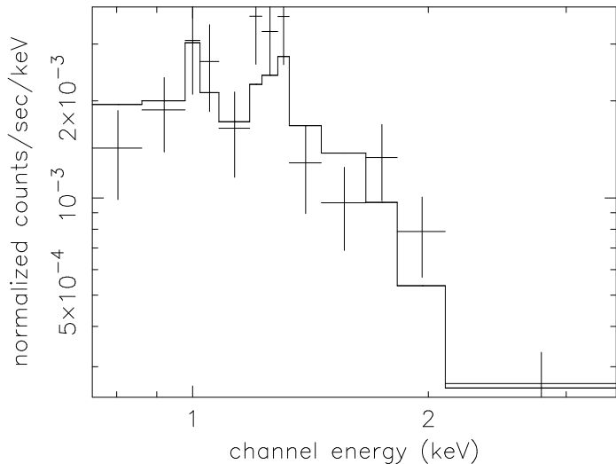
Fig. 10.— ACIS-I Spectra of the southwest, together with the best-fit thermal plasma spectral model (see text for details). The on-source spectral data were extracted from the ellipse outlined in Fig. 2 (see also §2).
