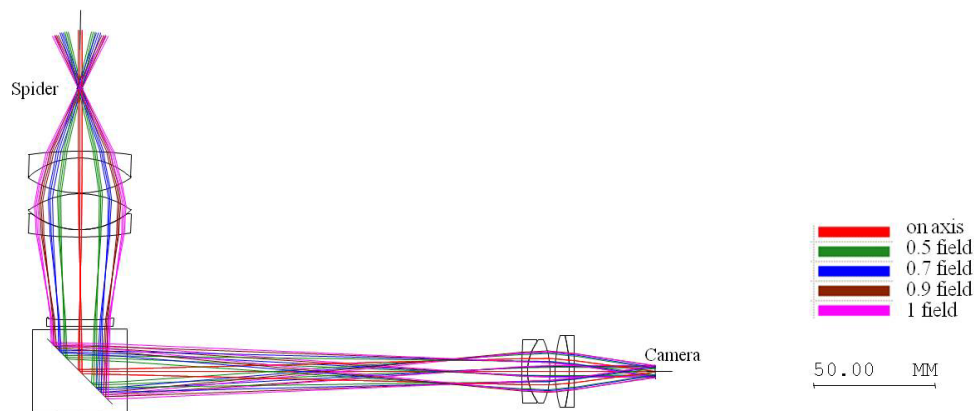
Figure 7. Retinal imaging sub-system.
