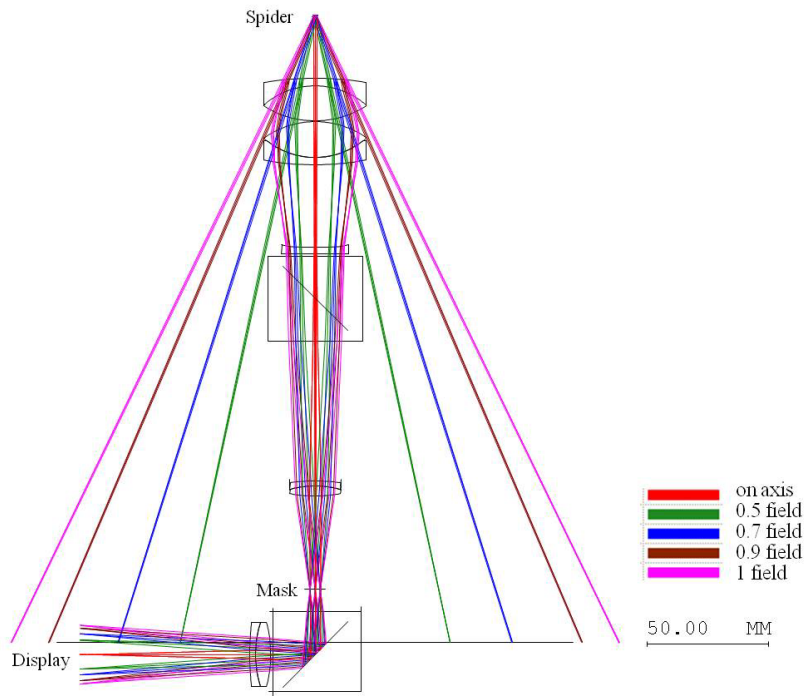
Figure 3. Stimuli presentation sub-system.
