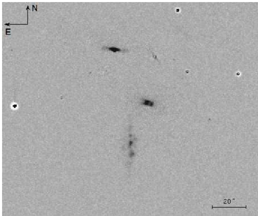
Fig. 9.— Continuum-subtracted H_{\alpha} interference filter image centered at 6667 Å of SS.
