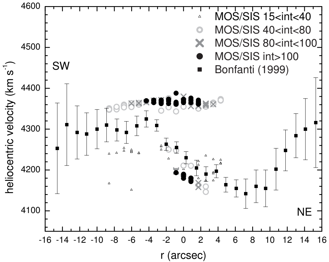
Fig. 11.— H79a line of sight velocity curve along major axis ( \text{PA}=65^\circ ). "int" corresponds to the intensity of the peak of each component.
